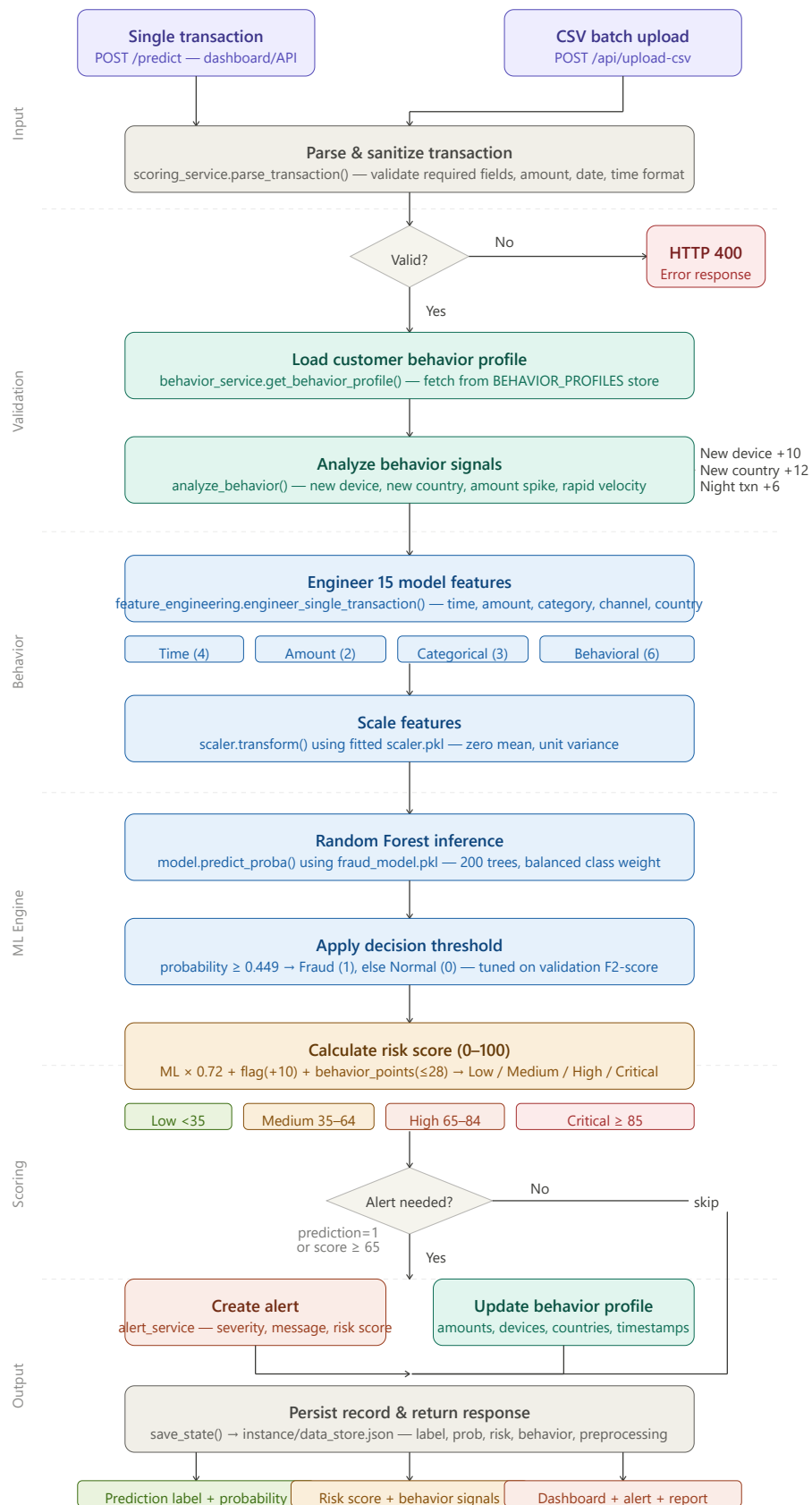
Figure 4.1: Prediction Workflow Flowchart
