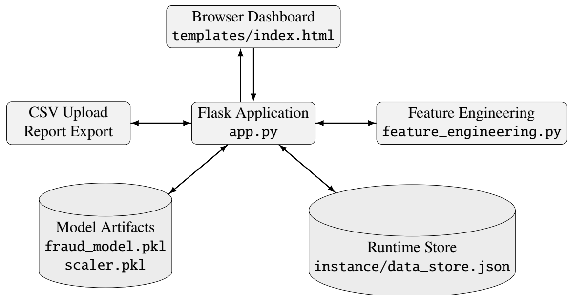
Figure 5.1: System Architecture
