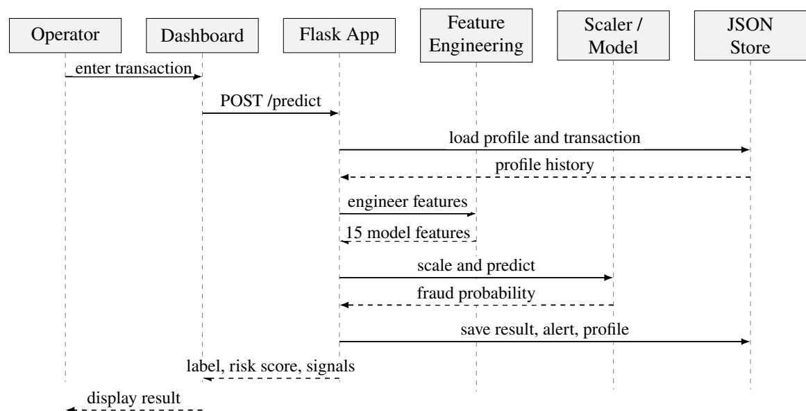
Figure 5.4: Single Transaction Prediction Sequence
