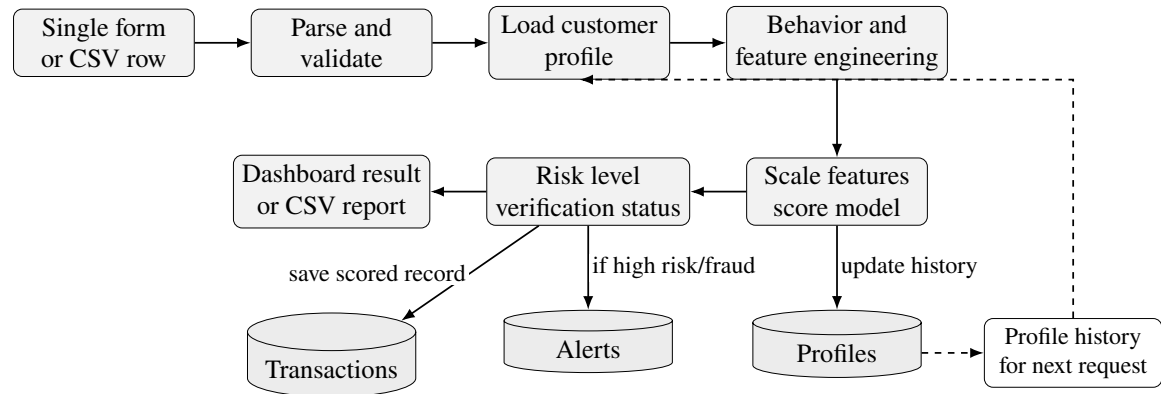
Figure 5.3: Transaction Data Flow
