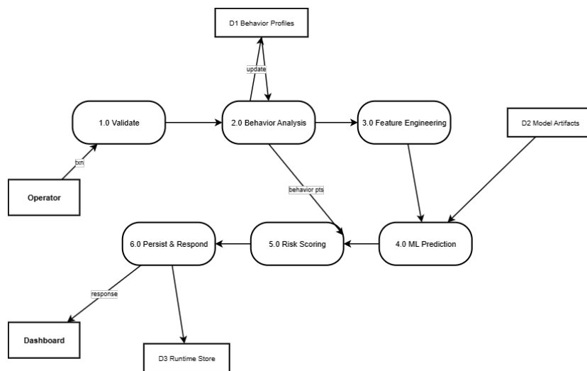
Figure 5.3: Data Flow Diagram
