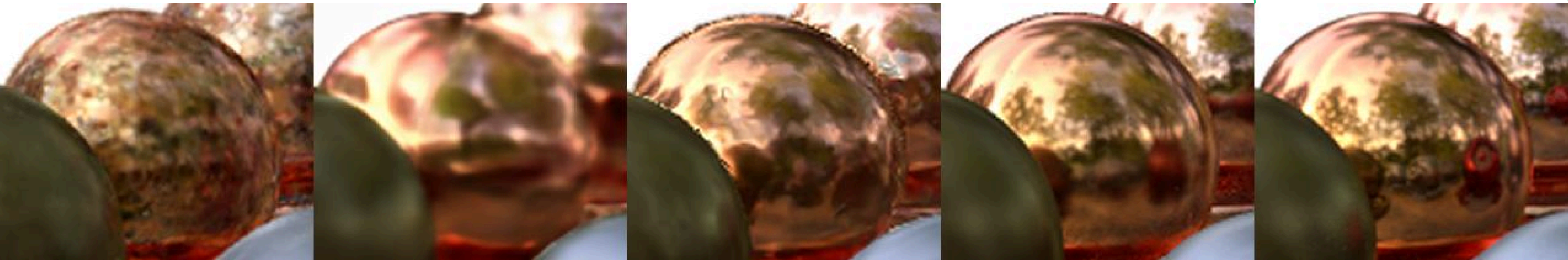
2DGS
