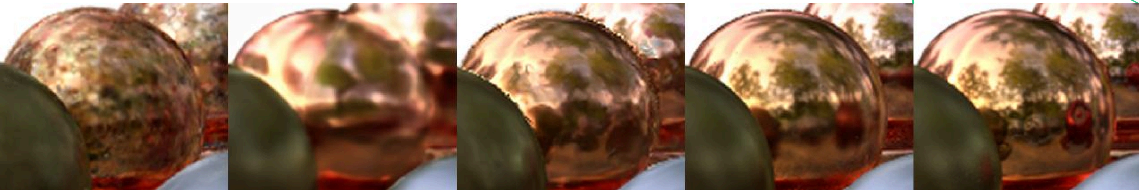
2DGS
