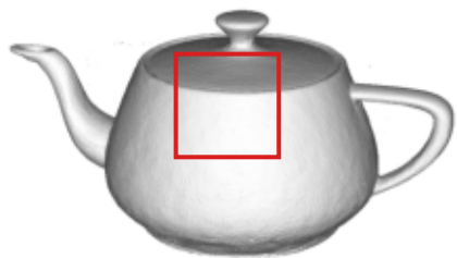
teapot view 58
