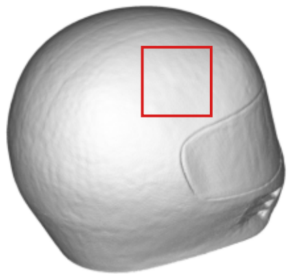
helmet view 143
