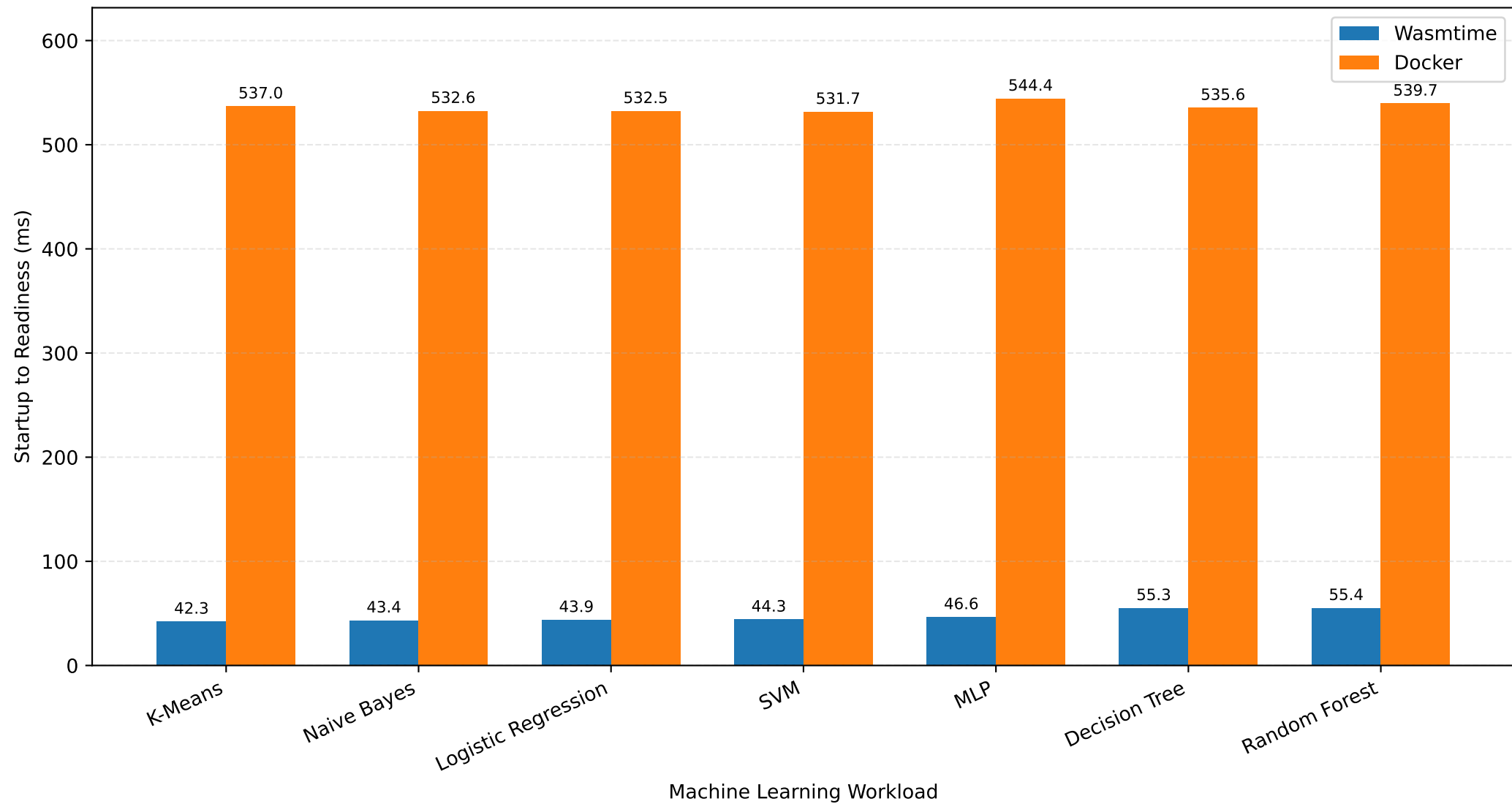
Cold-Start Readiness: Wasmtime vs Docker
