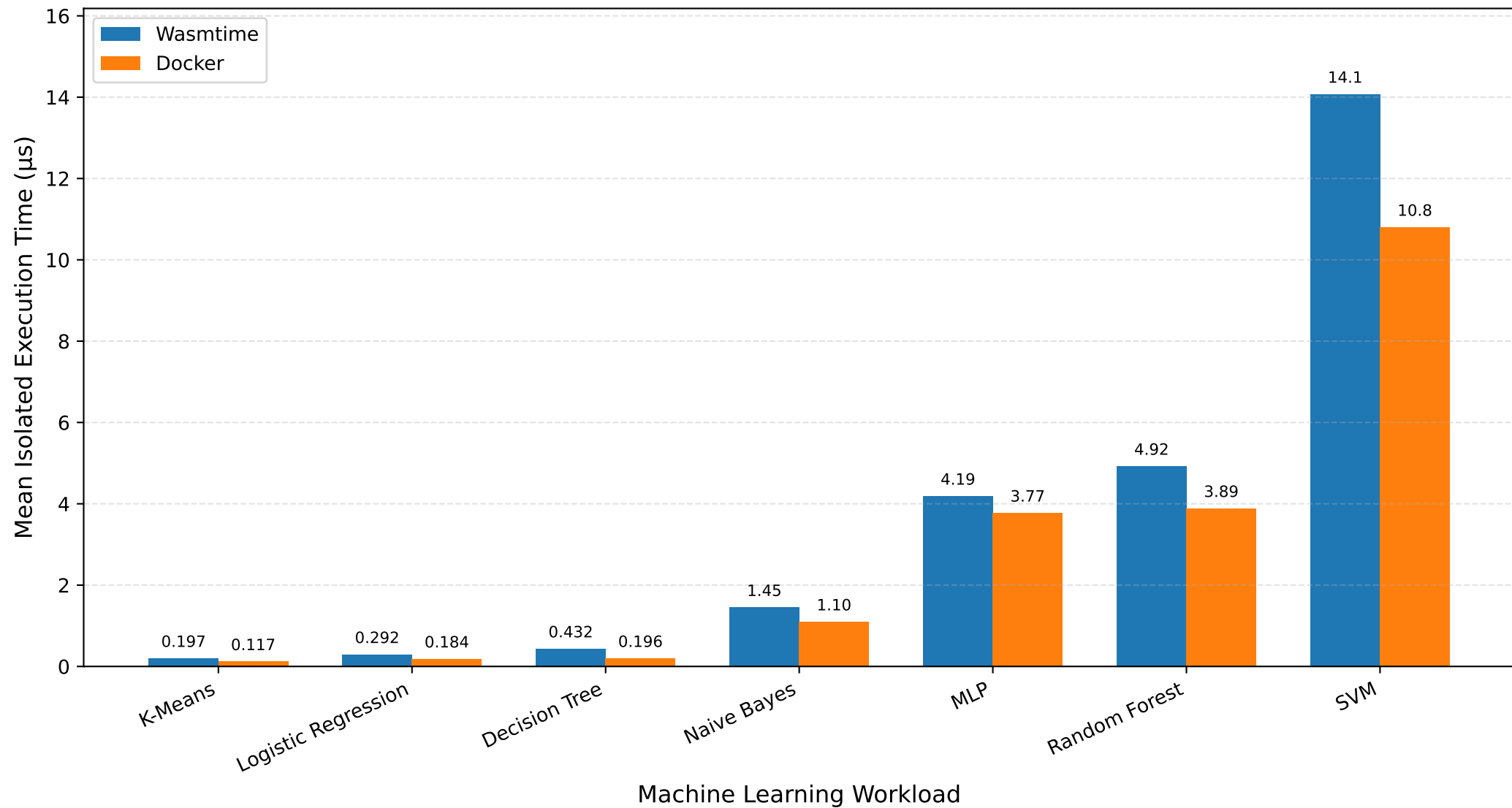
Isolated Model Execution Time: Wasmtime vs Docker
