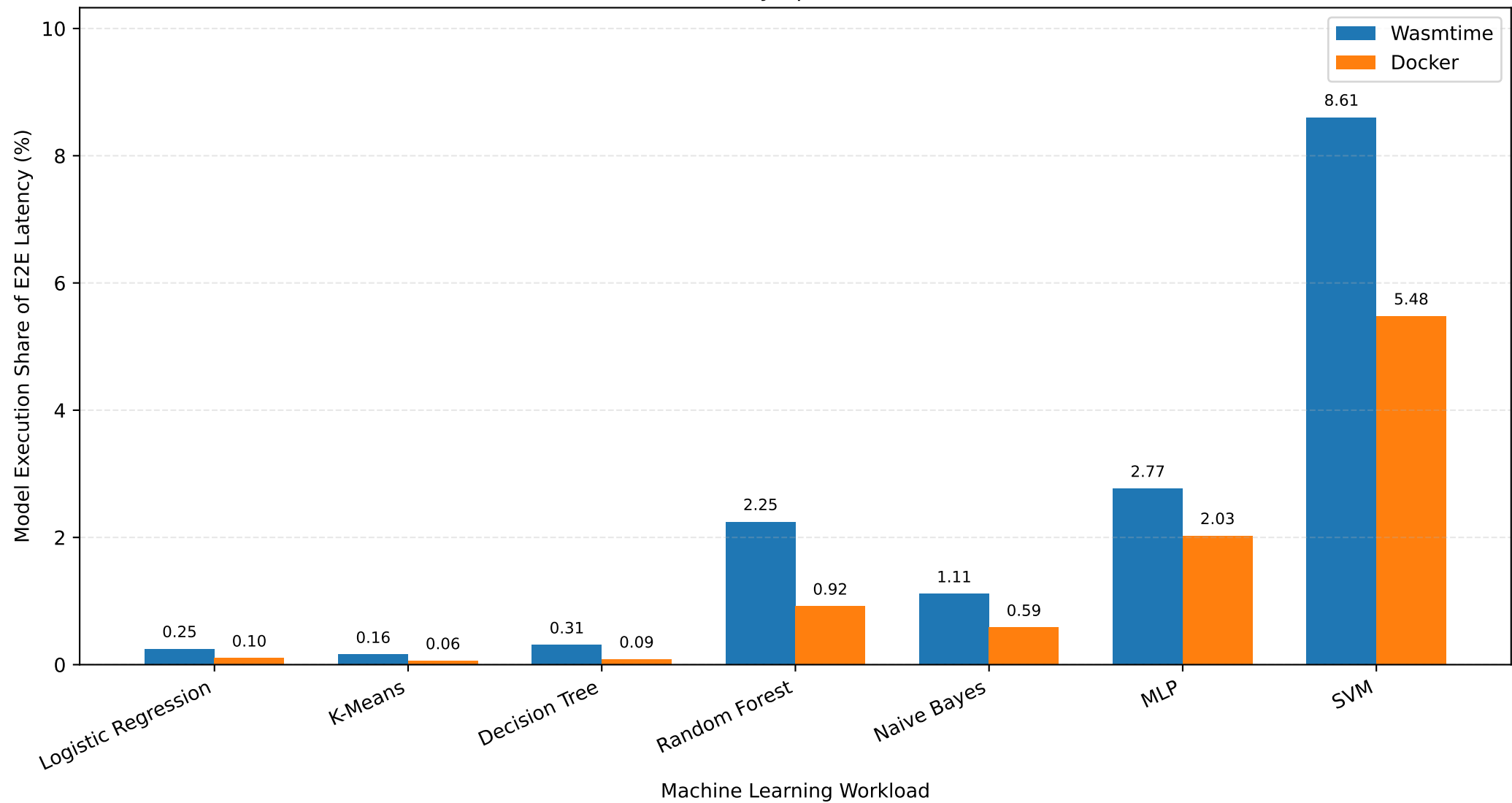
Fraction of End-to-End Latency Spent in Isolated Model Execution
