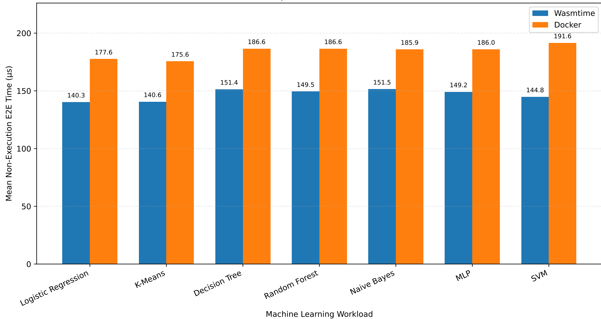
End-to-End Latency Outside Isolated Model Execution
