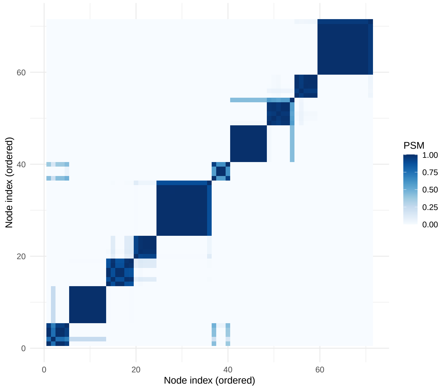
PSM (ordered by VI partition) – best by cov silhouette: (1.00, 2.00, 1.00)
