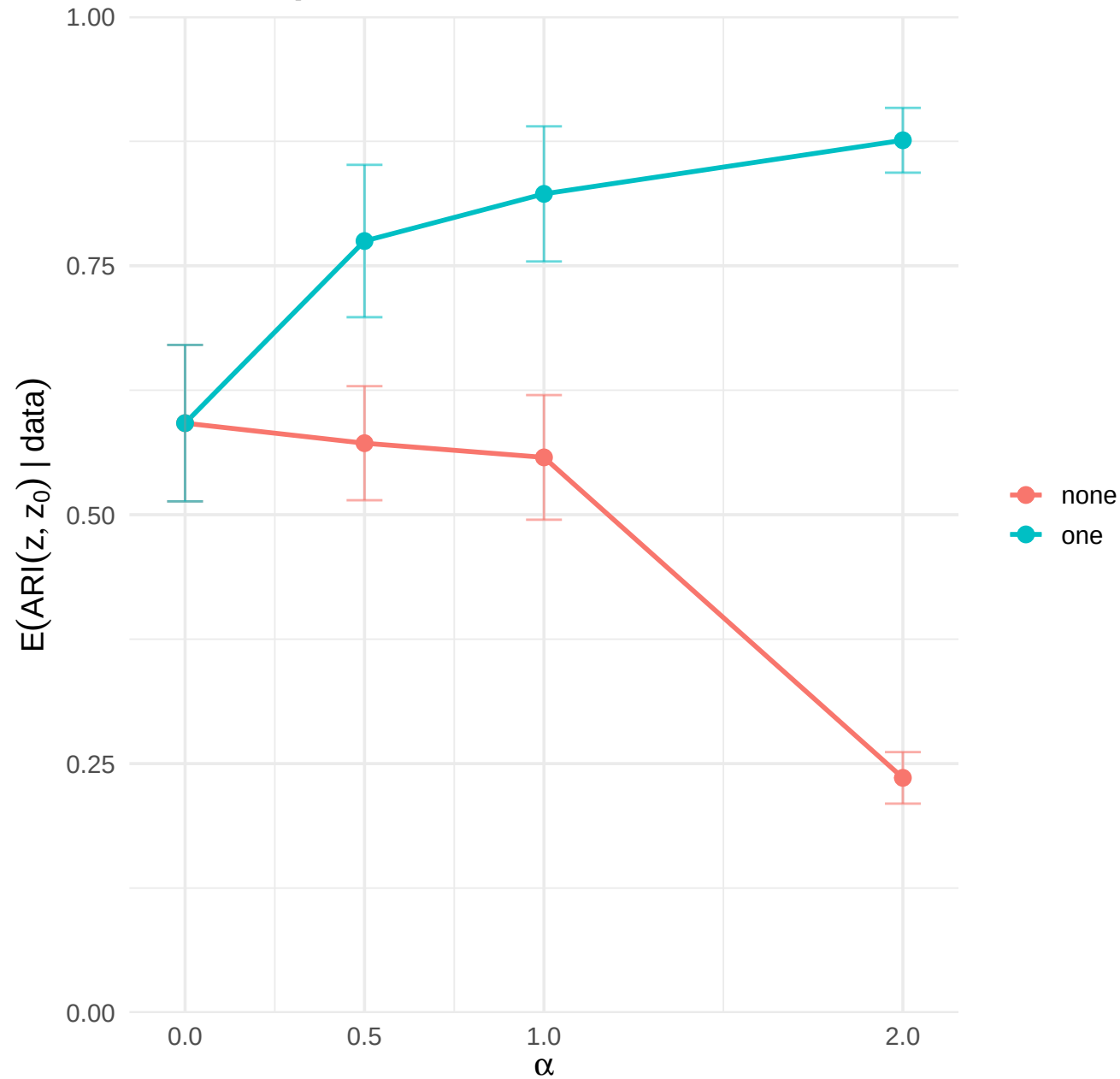
ARI vs alpha
