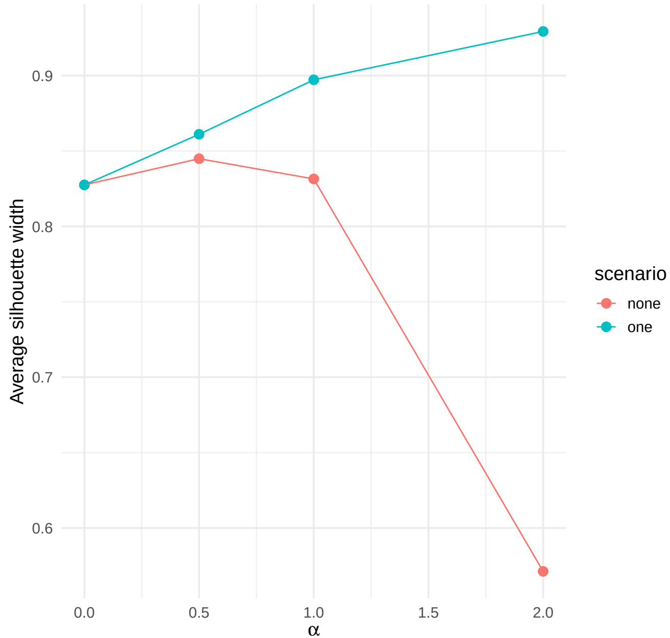
Silhouette vs alpha
