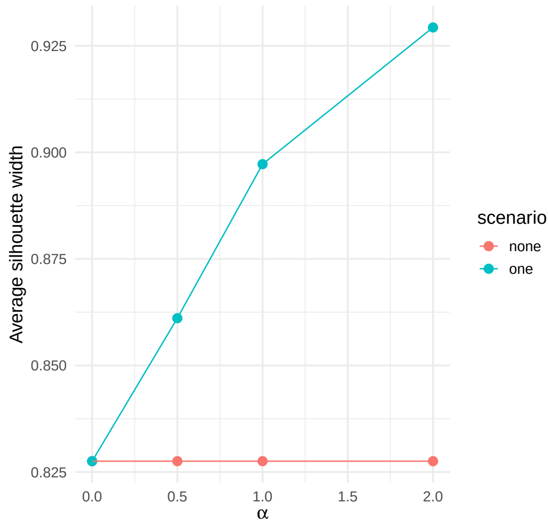
Silhouette vs alpha
