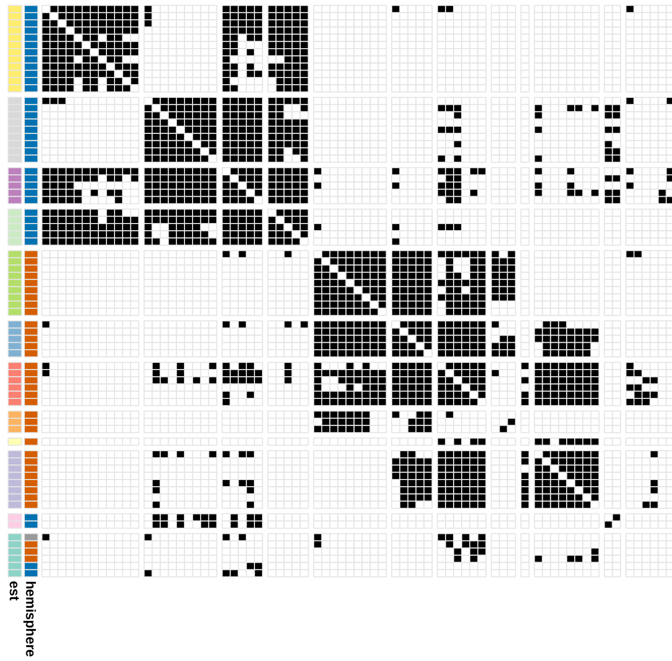
Adjacency , \alpha=(0.00,0.00,0.00)
