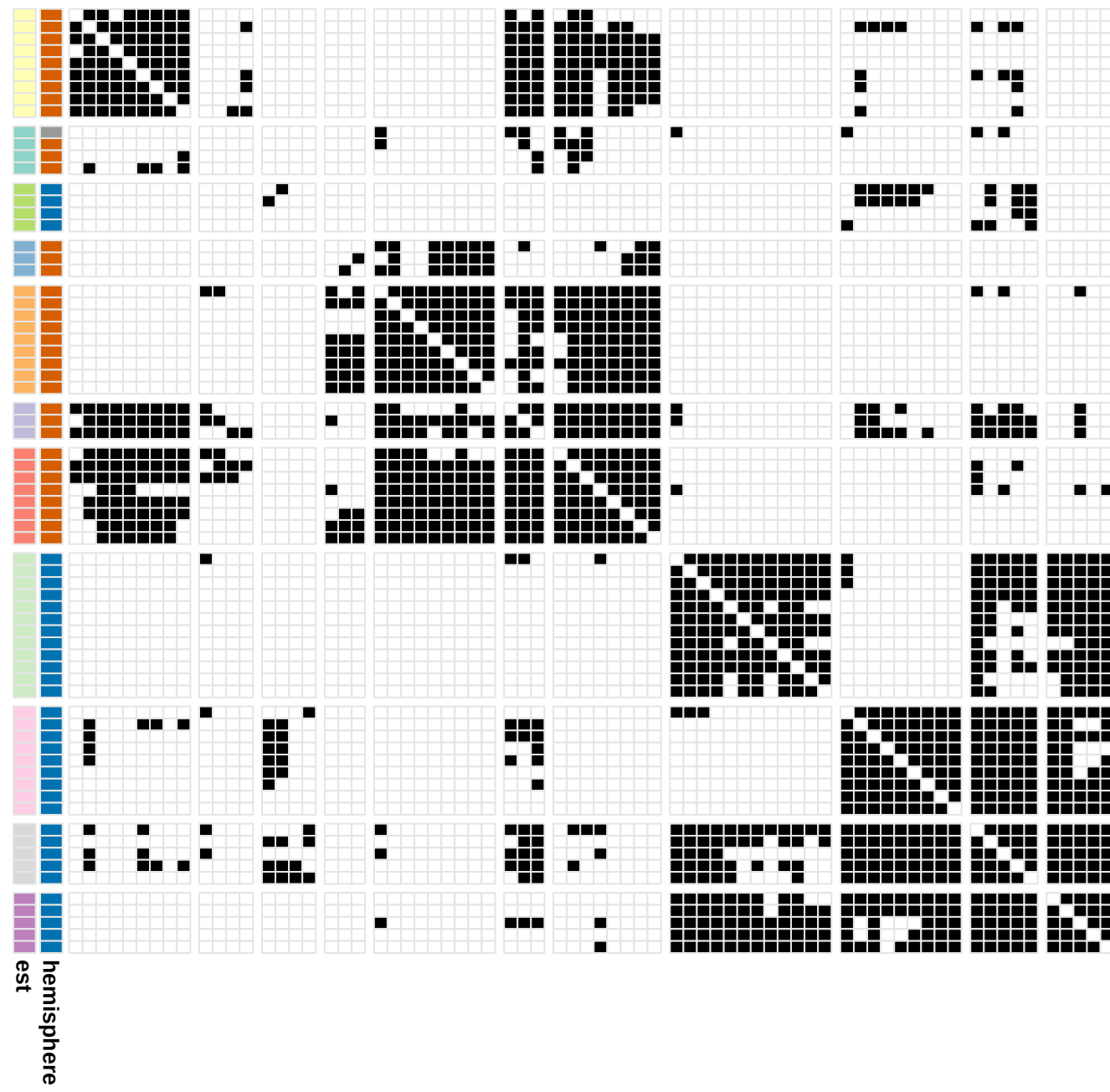
Adjacency , alpha=(2.00,0.00,0.00)
