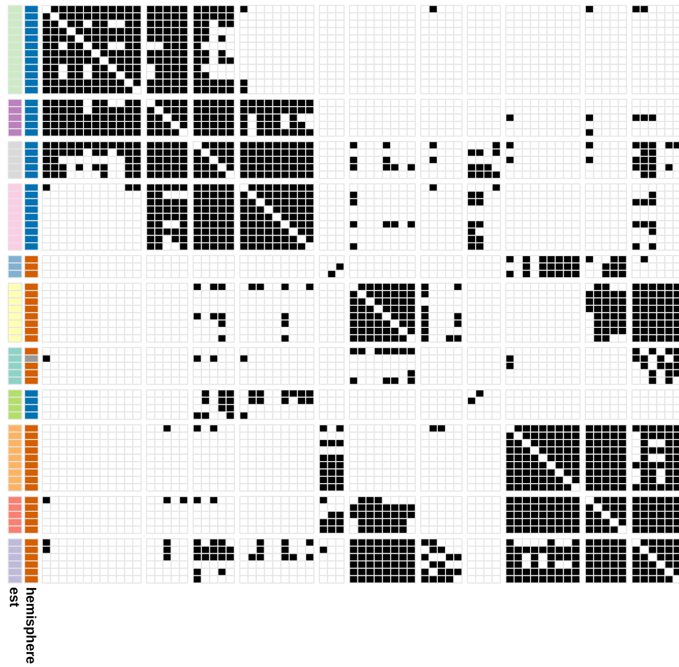
Adjacency , alpha=(0.00,1.00,0.00)
