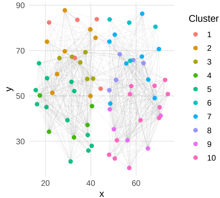
VI clusters, \alpha=(0.00,2.00,0.00) , K_{\text{hat}}=10
