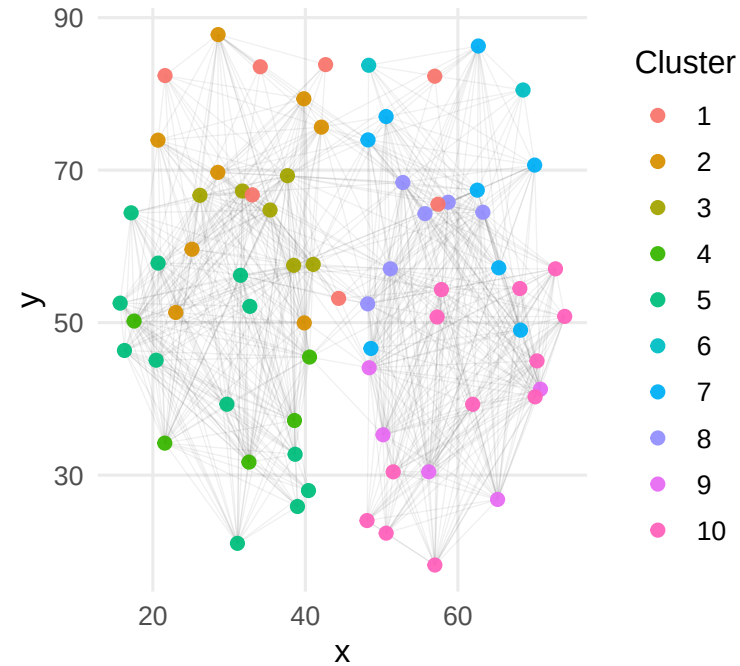
VI clusters, \alpha=(0.00,0.00,2.00) , K_{\text{hat}}=10
