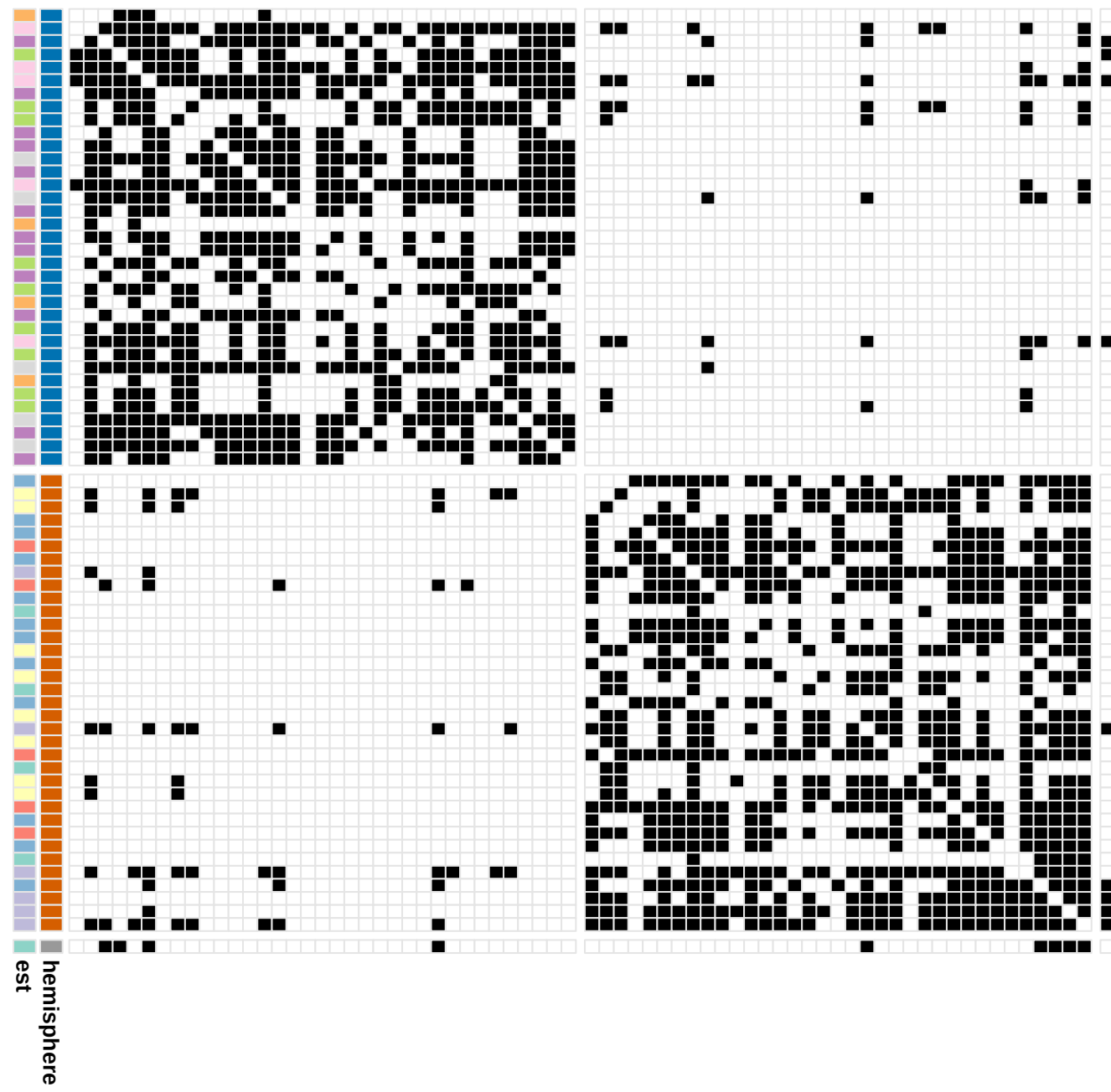
Adjacency (Left-Right order), alpha=(0.00,2.00,0.00)
