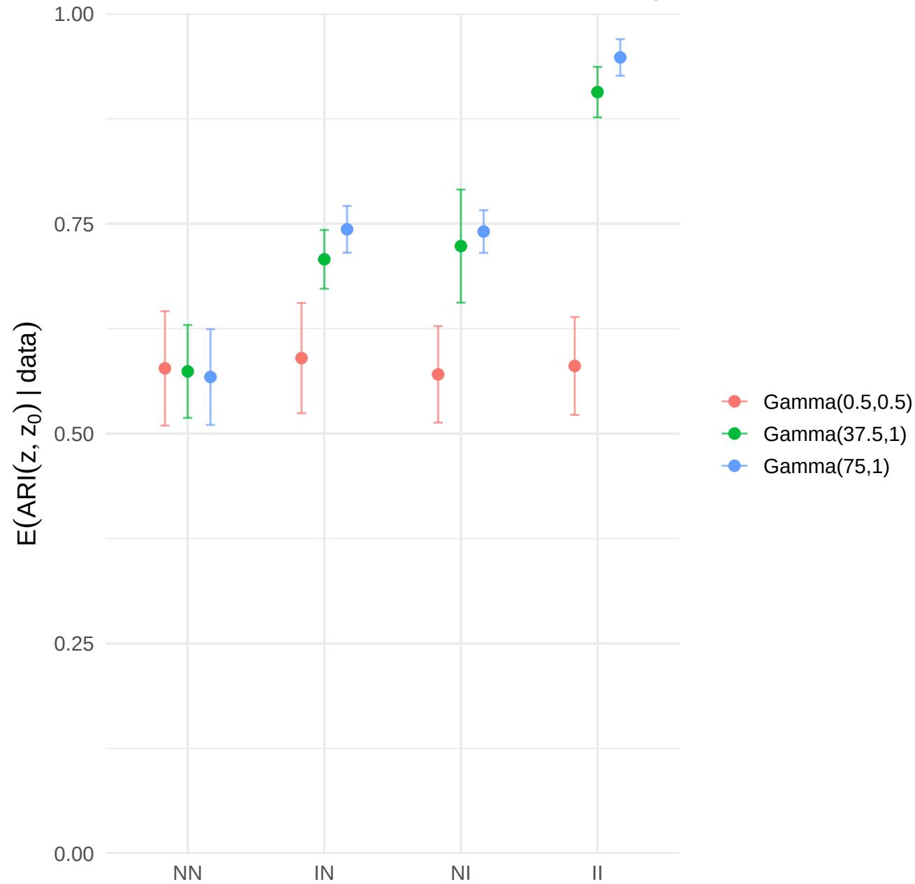
Posterior mean ARI under learned alpha
