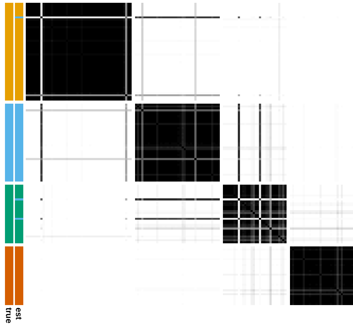
Informative covariate (alpha = 2)
