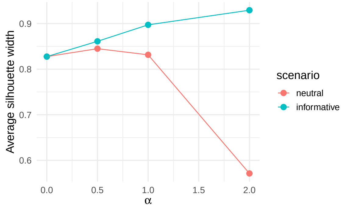
Silhouette vs alpha
