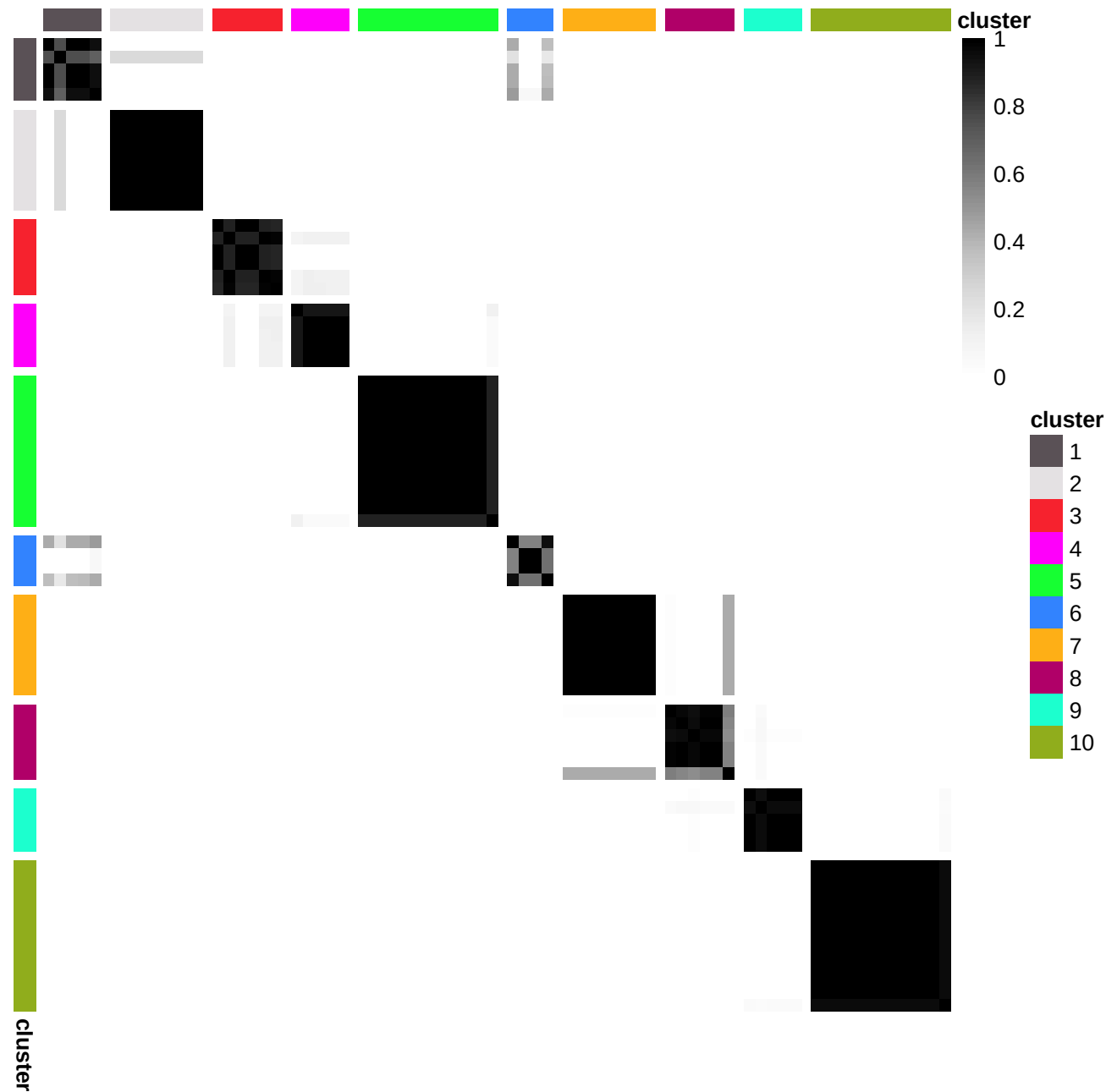
PSM – best by cov silhouette
