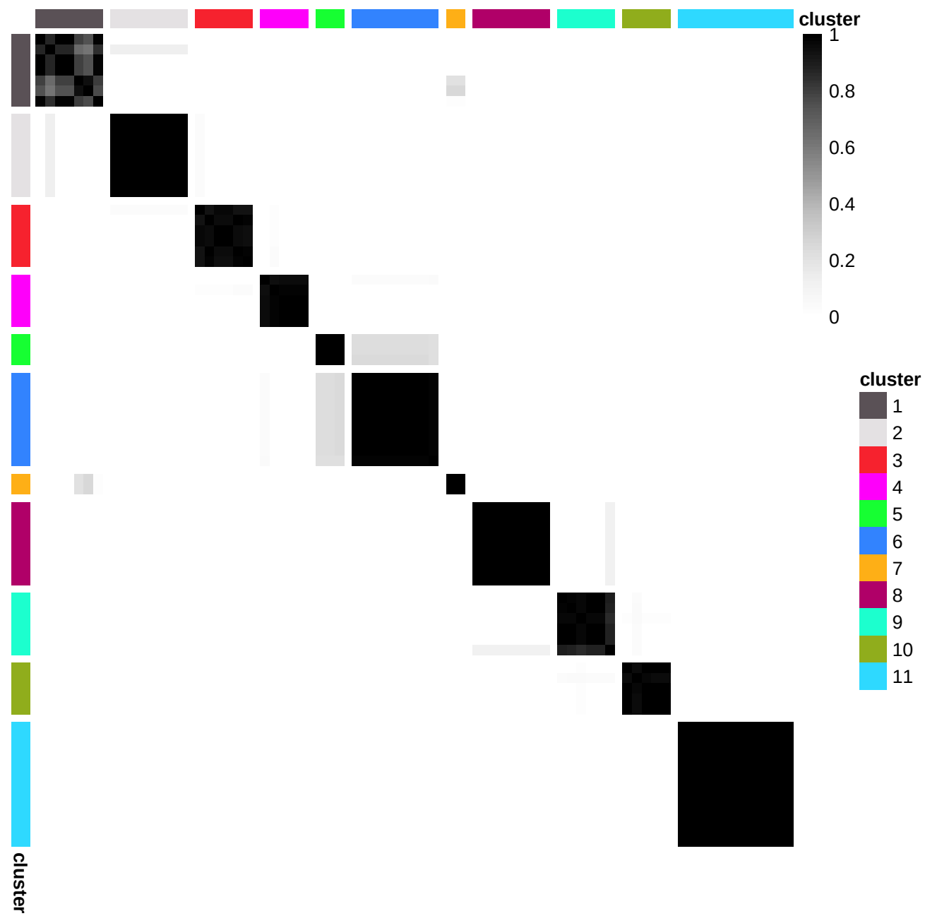
PSM – best by post silhouette
