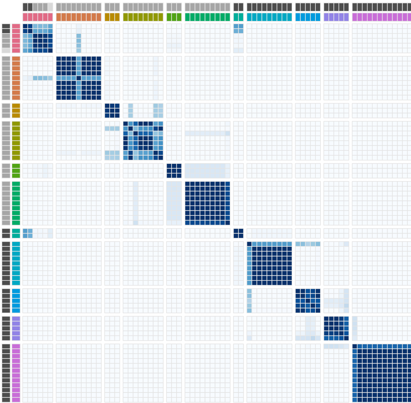
PSM, alpha=(1.00,0.00,0.00), K_hat=11
