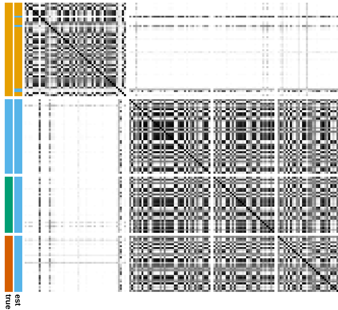
Covariate effect ( \alpha = 2 )
