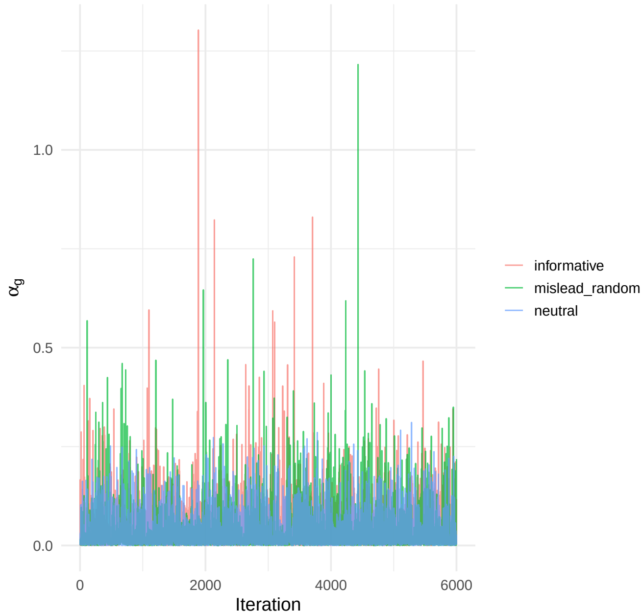
Trace plots for learned alpha
