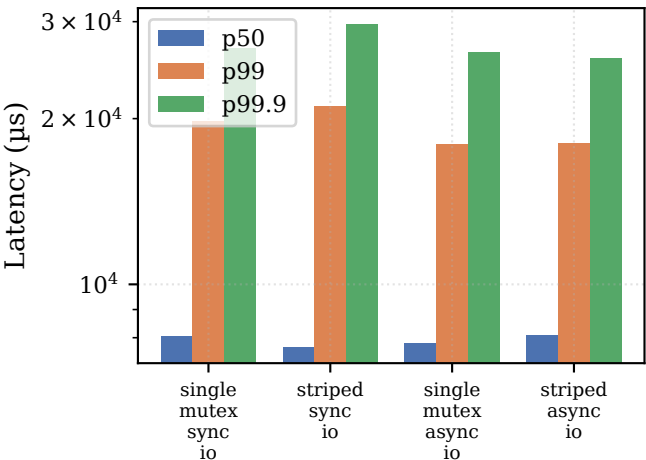
Ablation: tail latency across LSM configurations
