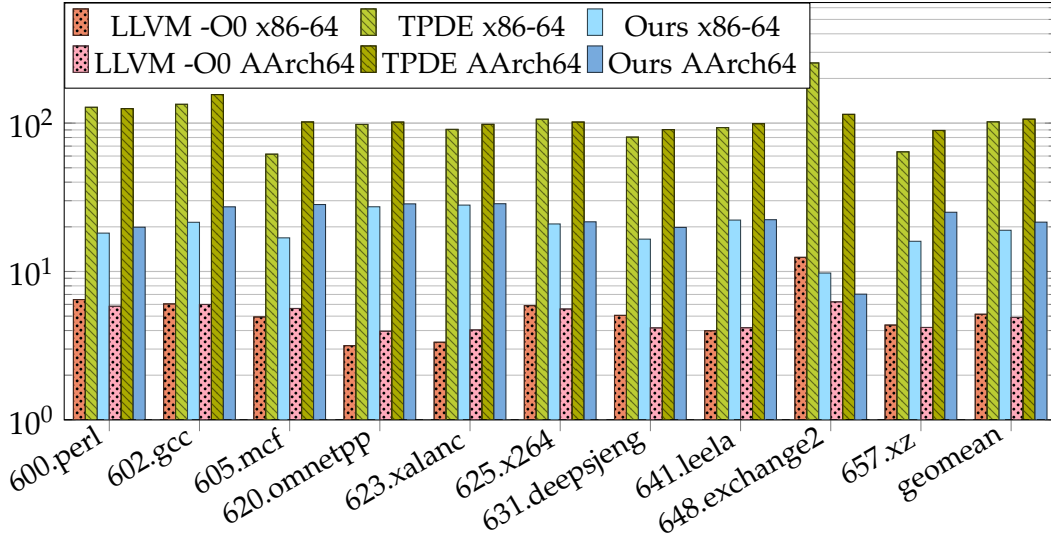
Figure 5.2: SPEC CPU2017 integer compile time speedup relative to LLVM-O1 backend with optimized IR. (log scale)
