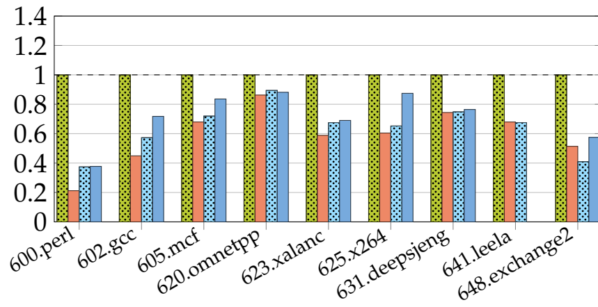
Figure 5.1: SPEC CPU2017 integer runtime speedup relative to clang-O1. Values are derived from the raw ‘res-spec-raw-rt’ data. Missing measurements are omitted. On AArch64, the available clang runtime file is reused as the comparison baseline because no separate clang-O1 runtime file is present in the data.
