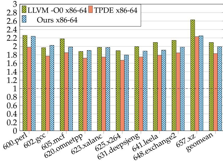
Figure 5.4: SPEC CPU2017 integer text size relative to clang-O1 backend with optimized IR.
