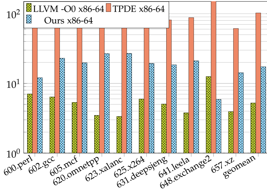
Figure 5.3: SPEC CPU2017 integer compile time speedup relative to clang-O1 backend with optimized IR. (log scale)
