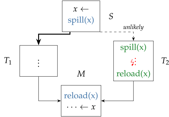
Figure 4.2: Example of a bad case for our simplified analysis. Green represents the ideal spill and reload locations. Blue is our approximation. T_2 is assumed to have high register pressure, therefore x has to be spilled. We assume that the branch to T_2 is unlikely, therefore we generate unnecessary spills and reloads.
