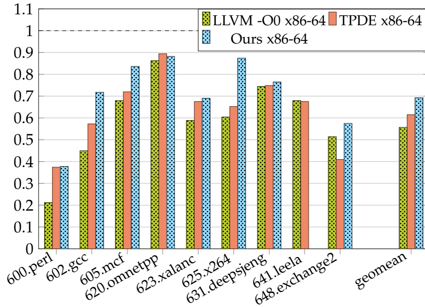
Figure 5.1: SPEC CPU2017 integer runtime speedup relative to clang-O1 backend with optimized IR.
