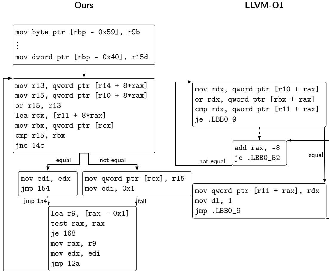
Figure 5.2: Example of a small loop from bitmap_elt_ior , one of the critical functions of 602.gcc . Generated by our implementation and llvm-O1 . We can clearly see a better instruction selection and more optimizations such as the loop counter.
