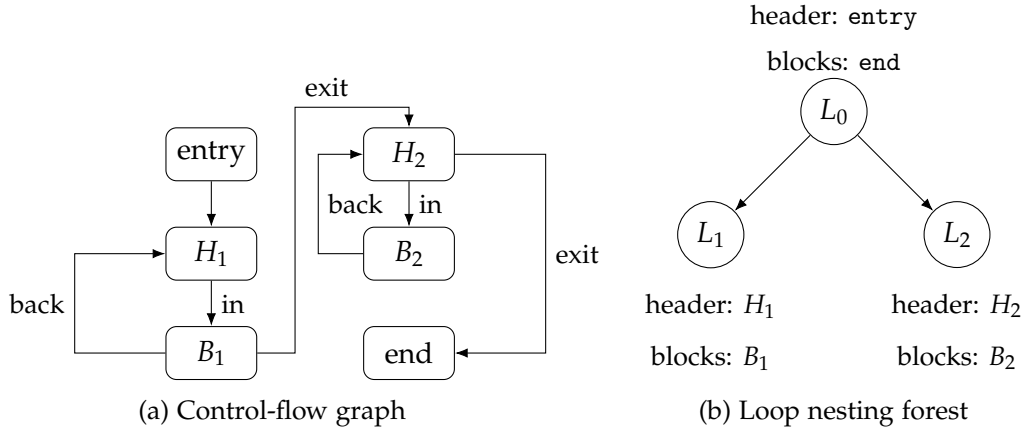
Figure 4.1: A control-flow graph and its corresponding loop nesting forest [Boi+11]. The outermost loop L_0 is only the root of the tree, and does not get treated as a loop, this corresponds to the existing loop analysis in TPDE [SKE25]. The edges marked in and back are loop edges, along which the header liveness is propagated. On edges marked exit the loop exit penalty is added if a value is live after the loop.
