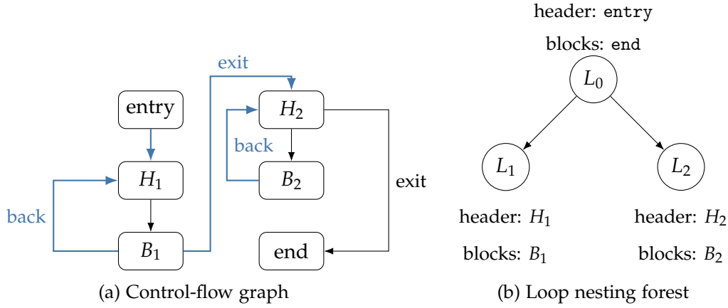
Figure 3.1: A control-flow graph and its corresponding loop nesting forest [Boi+11]. The outermost loop L_0 is only the root of the tree, and does not get treated as a loop, this corresponds to the existing loop analysis in TPDE [SKE26]. The edges marked blue are loop edges, as they connect to a loop header, which are skipped on the partial liveness pass. On edges marked exit the loop exit penalty is added if a value is live after the loop.
