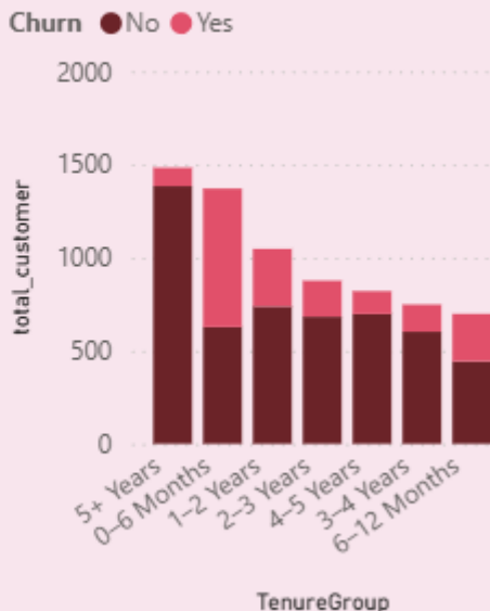
Customer Churn by Tenure Group
