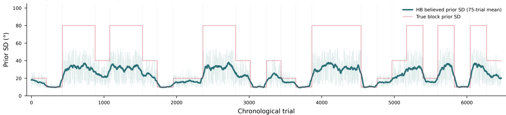
Participant 12 — HB learned prior confidence tracks block width
