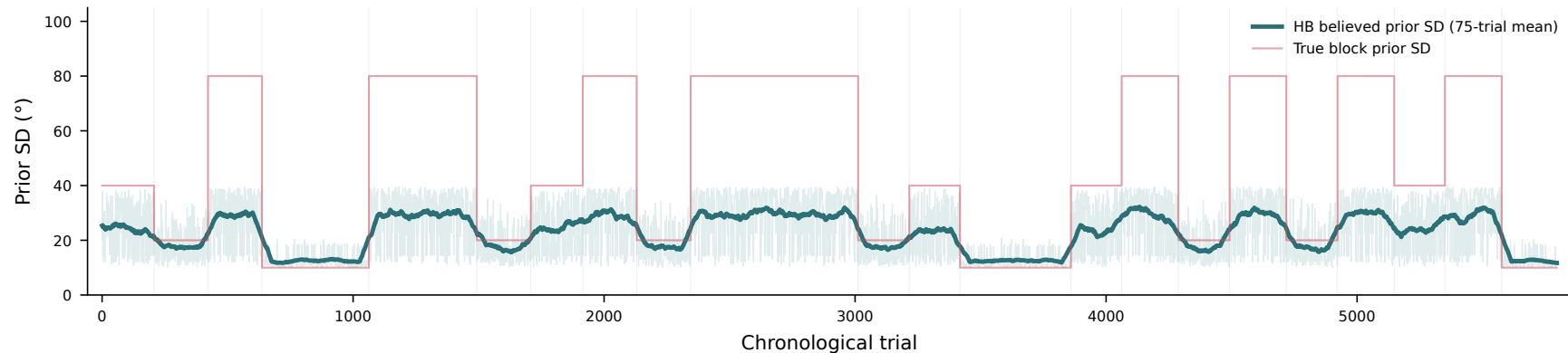
Participant 8 — HB learned prior confidence tracks block width
