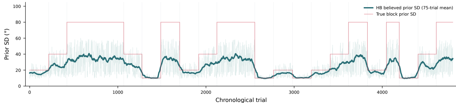
Participant 4 — HB learned prior confidence tracks block width
