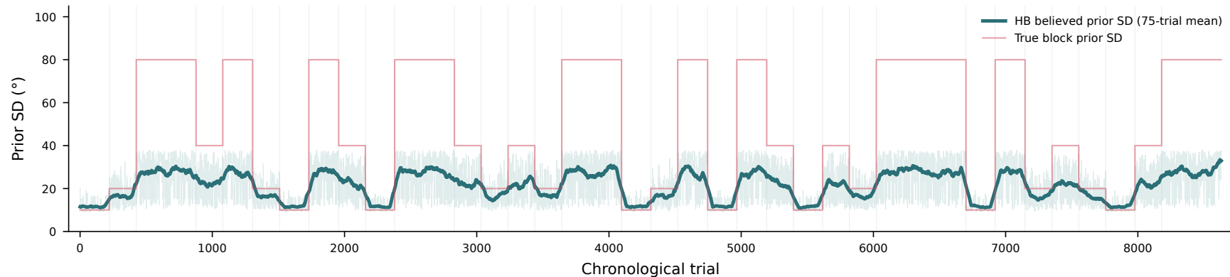
Participant 9 — HB learned prior confidence tracks block width
