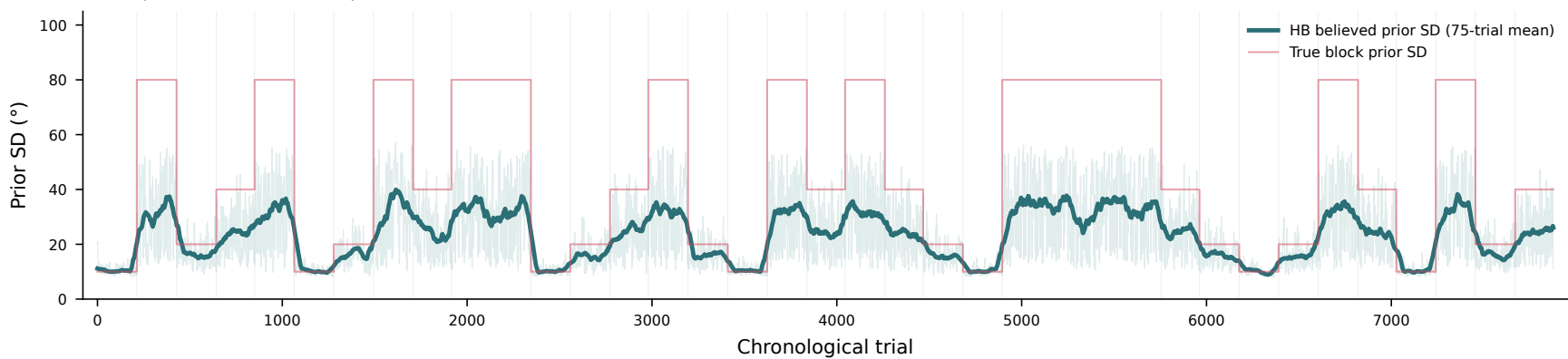
Participant 2 — HB learned prior confidence tracks block width
