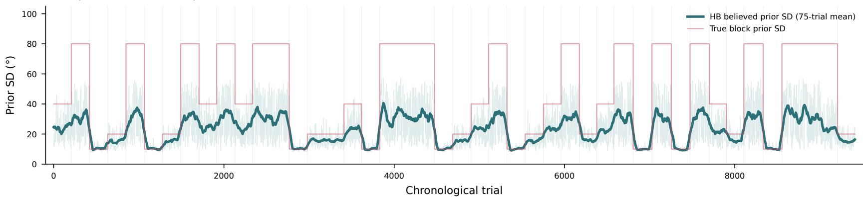
Participant 3 — HB learned prior confidence tracks block width
