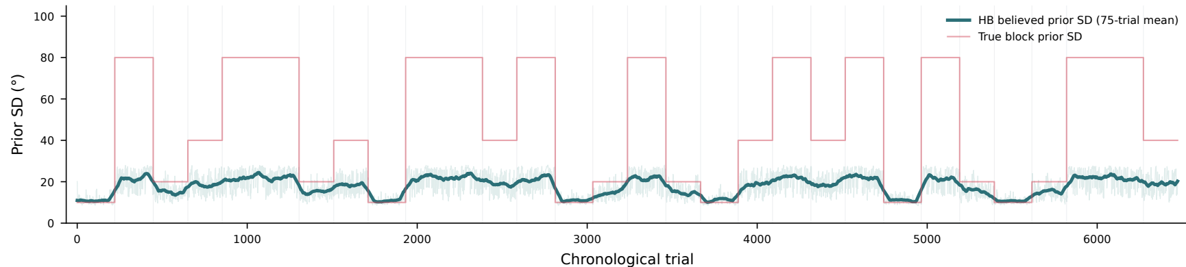
Participant 11 — HB learned prior confidence tracks block width
