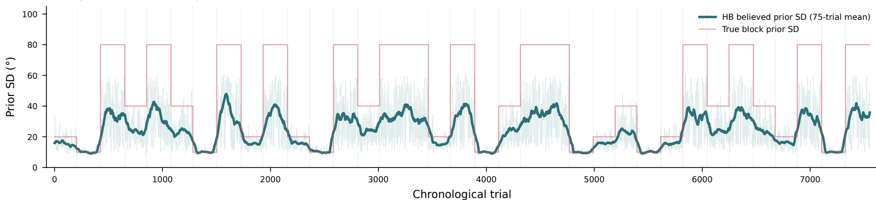
Participant 6 — HB learned prior confidence tracks block width
