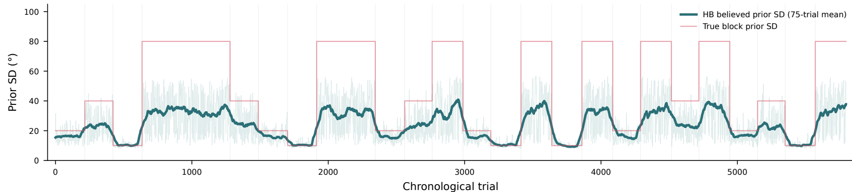
Participant 7 — HB learned prior confidence tracks block width
