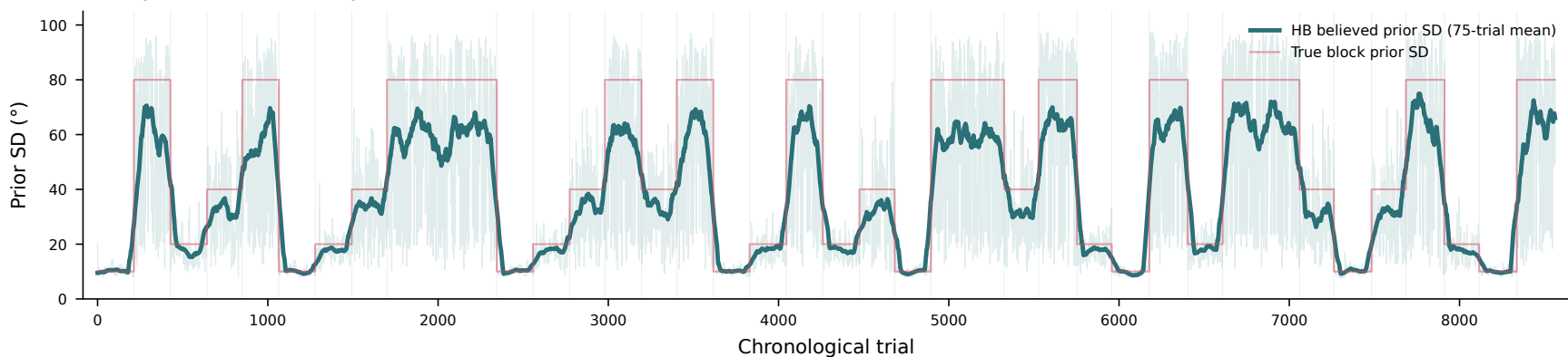
Participant 1 — HB learned prior confidence tracks block width
