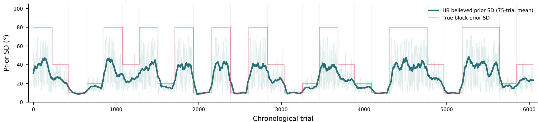
Participant 10 — HB learned prior confidence tracks block width
