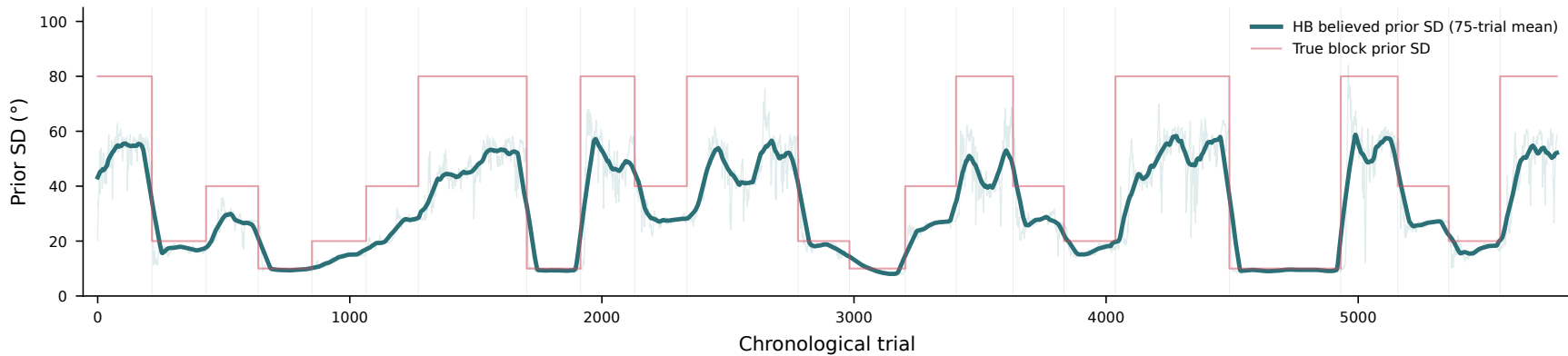
Participant 5 — HB learned prior confidence tracks block width
