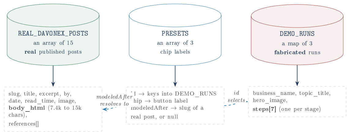
Figure 4: The three constants and how they reference each other. PRESETS is the join table: it links a fabricated run to the real post whose shape inspired it.
