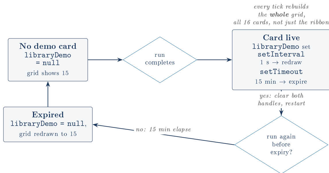
Figure 7: The demo card’s lifetime. The re-run path is handled correctly: both the interval and the timeout are cancelled before new ones are created, so timers cannot leak.
