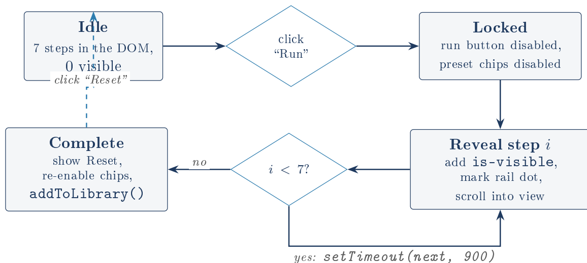
Figure 6: The run loop. All seven steps already exist in the DOM before the button is pressed; “running” only adds a CSS class to one more of them every 900 ms.
