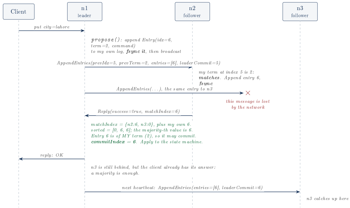
Figure 8: The replication path for one write. The client is answered as soon as a majority has the entry stored durably; the straggler catches up on the next heartbeat. Losing n3’s message costs nothing, because AppendEntries is idempotent and heartbeats retry forever.
