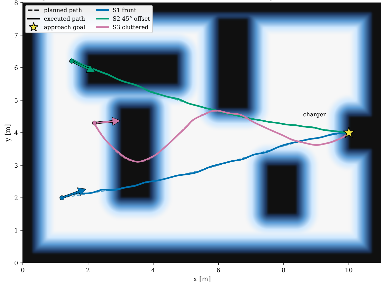
Navigation costmap with planned (- -) and executed (—) trajectories
