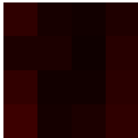
Quantum Recon
