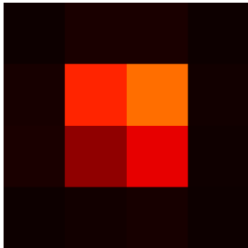
Classical Recon
