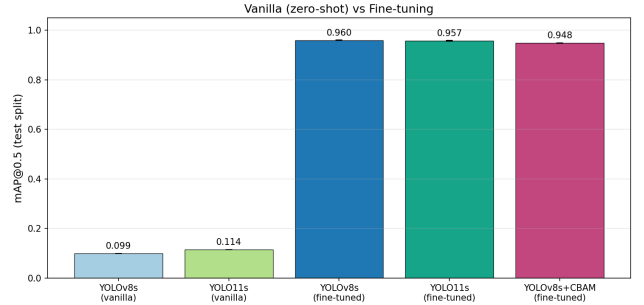
Fig. 2. Accuracy jump from the zero-shot baseline (about 0.10) to the fine-tuned models (about 0.96) on mAP@0.5. The difference among architectures after fine-tuning is far smaller than the effect of fine-tuning itself.
