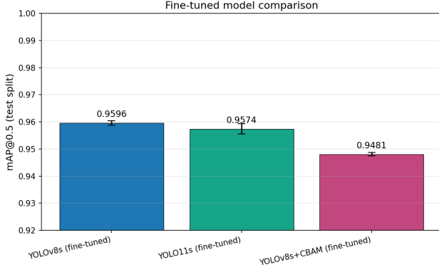
Fig. 3. mAP@0.5 across the three fine-tuned architectures (mean \pm std, n = 3 ). YOLOv8s leads slightly on mAP@0.5; on mAP@[.5:.95] the order changes (YOLO11s highest, Table III).
