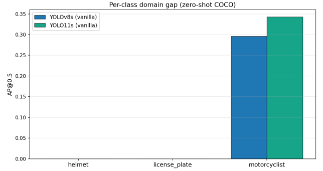
Fig. 1. Per-class AP@0.5 under zero-shot COCO. The helmet and license-plate classes are zero by design (no COCO counterpart); only the motorcyclist class receives a signal through the mapping from COCO motorcycle.
