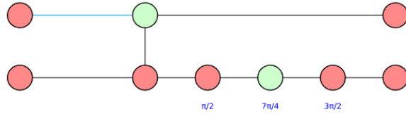
Figure 15: ZX diagram corresponding to (x, y) = (0, 0) and (m_0, m_1) = (0, 0)
