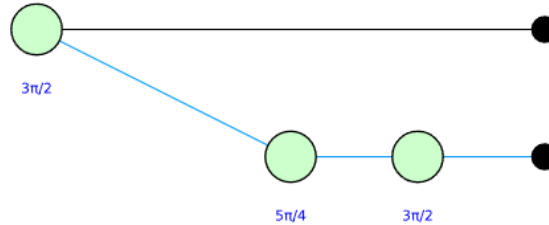
Figure 17: Simplification of the ZX diagram for the implementation of CHSH game, corresponding to (x, y) = (0, 0) .
