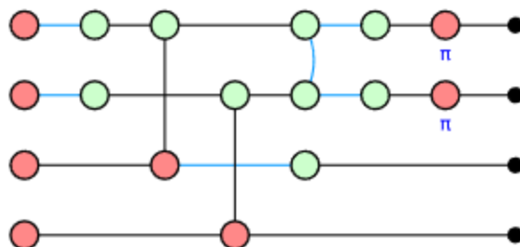
Figure 20: ZX diagram corresponding to the circuit in figure 9.
