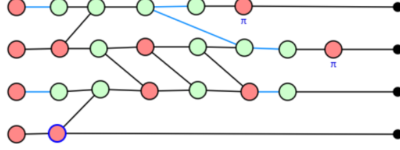
Figure 23: Visual representation of the orientation of edges for row 3 and column 0. Time flows from left to right.
