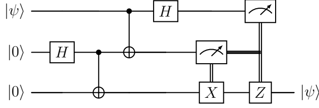
Figure 6: Standard quantum teleportation circuit.
