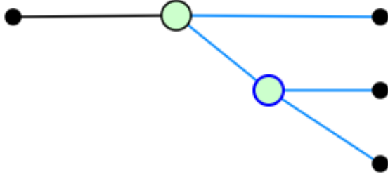
Figure 14: Simplified teleportation protocol without the classical control operations.
