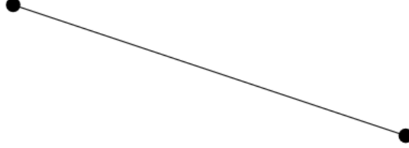
Figure 11: Identity channel resulting from the simplification of the teleportation diagrams
