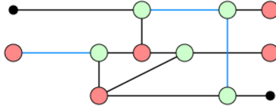
Figure 12: Simplification of the teleportation diagram when Alice measures (0, 0) .
