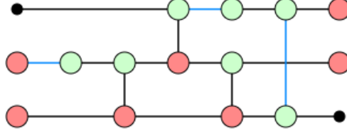
Figure 10: ZX diagram corresponding to a standard quantum teleportation when Alice measures (0, 0) .
