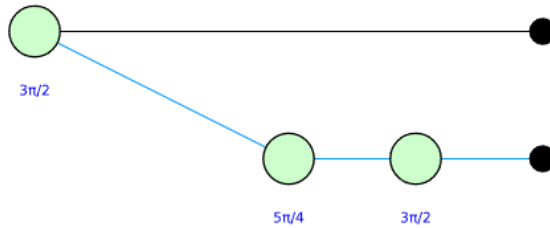
Figure 18: Simplification of the ZX diagram for the implementation of CHSH game, corresponding to (x, y) = (0, 0) .
