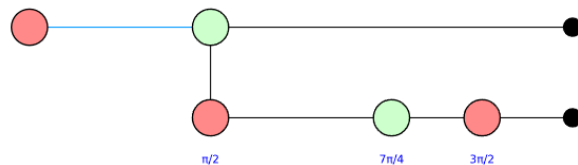
Figure 19: Simplification of the ZX diagram for the implementation of CHSH game, corresponding to (x, y) = (0, 0) , and with preparation of initial state in the computational basis.
