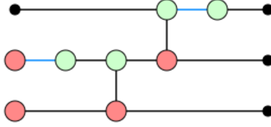
Figure 13: Teleportation protocol without the classical control operations.
