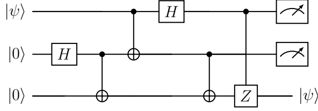
Figure 7: Standard quantum teleportation circuit without classical control.
