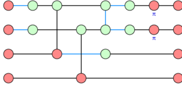
Figure 21: ZX diagram for row 3 and column 0 with boundary conditions corresponding to the covector \langle 0000| .
