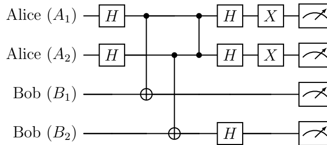
Figure 9: Mermin-Peres game circuit implementation for the first column and the third row.
