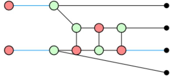
Figure 24: Simplified graph for row 3 and column 0.
