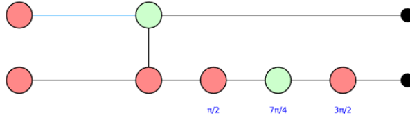
Figure 17: ZX diagram for the implementation of CHSH game, corresponding to (x, y) = (0, 0) .
