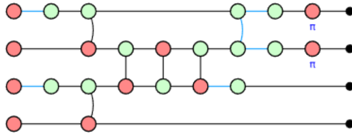
Figure 22: ZX diagram for row 3 and column 0 with 2DNN connectivity.
