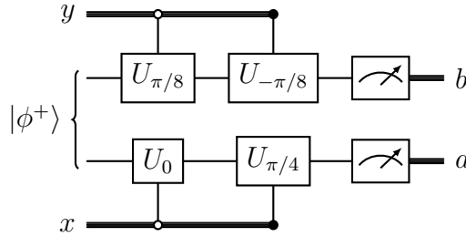
Figure 8: CHSH circuit for (x, y) = (0, 0)
