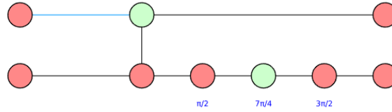
Figure 16: ZX diagram corresponding to (x, y) = (0, 0) and (m_0, m_1) = (0, 0)
