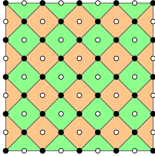
(a) A distance 5 planar surface code. Black dots represent data qubits, and white dots represent ancillary qubits. Green squares are X-type plaquettes stabilizers and orange squares are Z-type star stabilizers.
