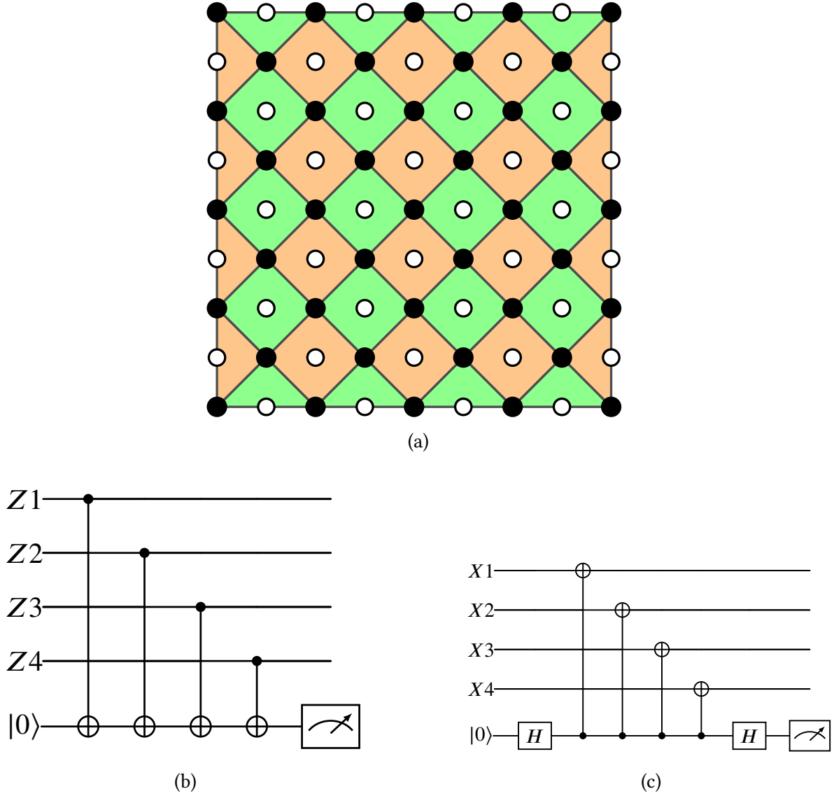
Figure 2.3: (a) A distance 5 planar surface code. Black dots represent data qubits, and white dots represent ancillary qubits. Green squares are X-type plaquettes stabilizers and orange squares are Z-type star stabilizers. (b) Z-syndrome. (c) X-syndrome.
