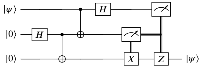
Figure 5.4: Standard quantum teleportation circuit.
