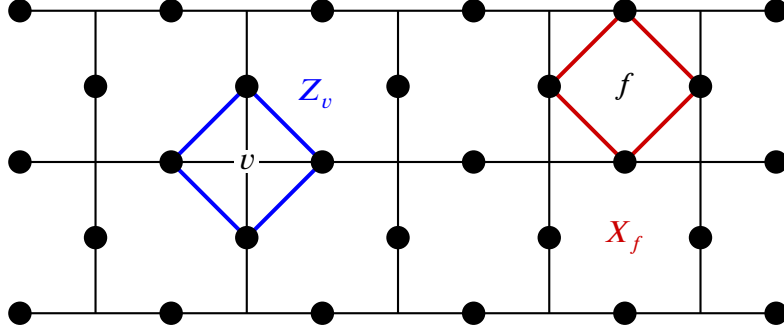
Figure 2.1: Lattice showing the arrangement of physical qubits and the support of the stabilizer generators.
