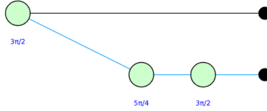
Figure 6.9: Simplification of the ZX diagram for the implementation of CHSH game, corresponding to (x, y) = (0, 0) .
