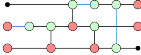
Figure 6.1: ZX diagram corresponding to a standard quantum teleportation when Alice measures (0, 0) .
