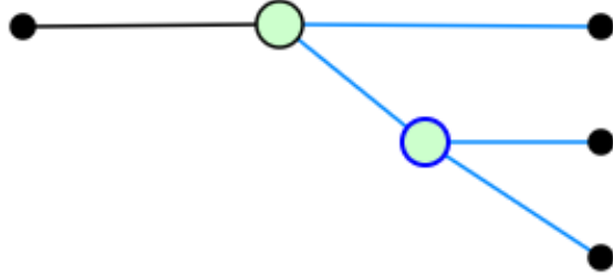
Figure 6.5: Simplified teleportation protocol without the classical control operations.
