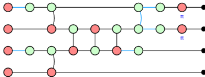
Figure 6.12: ZX diagram for row 3 and column 0 with 2DNN connectivity.
