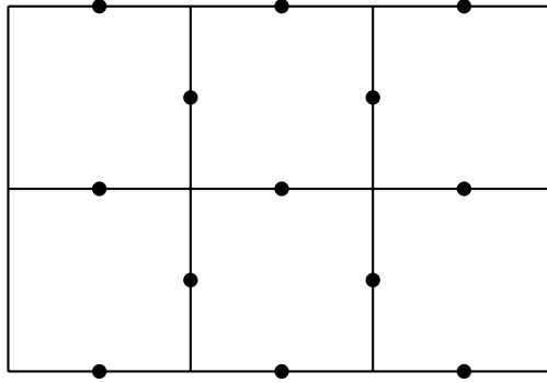
Figure 2.2: A planar patch. The top and bottom edges are closed (smooth) boundaries and the left and right edges are open (rough) boundaries. The black circles are once again physical qubits, and as we can see the open edges are not associated with any physical qubit.
