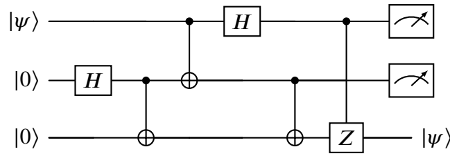
Figure 5.5: Standard quantum teleportation circuit without classical control.
