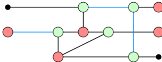
Figure 6.3: Simplification of the teleportation diagram when Alice measures (0, 0) .
