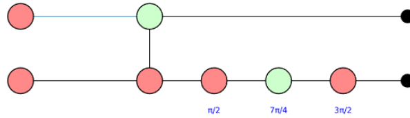
Figure 6.8: ZX diagram for the implementation of CHSH game, corresponding to (x, y) = (0, 0) .
