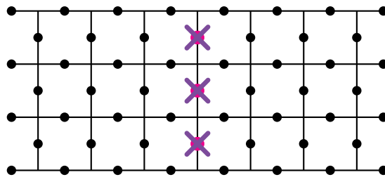
Figure 3.2: Physical distribution of qubits for a rough lattice splitting operation.
