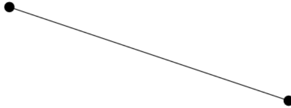
Figure 6.2: Identity channel resulting from the simplification of the teleportation diagrams
