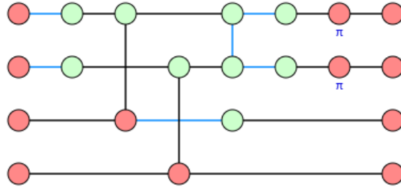
Figure 6.11: ZX diagram for row 3 and column 0, representing the circuit in 5.7, with boundary conditions corresponding to the covector \langle 0000| .
