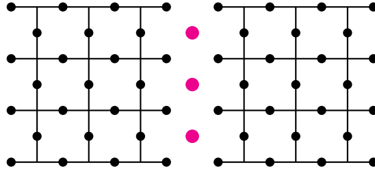
Figure 3.1: Physical distribution of qubits for a rough lattice merging operation. Black dots represent physical qubits subject to the stabilizers of their corresponding patch, and pink qubits are uninitialized physical qubits.
