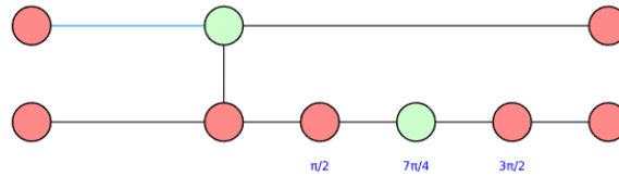
Figure 6.7: ZX diagram corresponding to (x, y) = (0, 0) and (m_0, m_1) = (0, 0)
