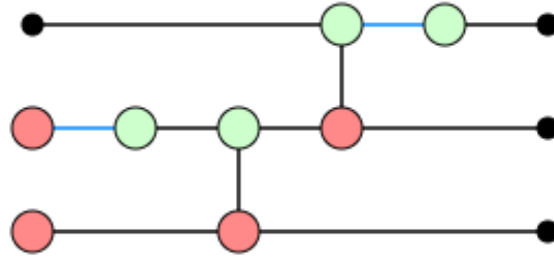
Figure 6.4: Teleportation protocol without the classical control operations.
