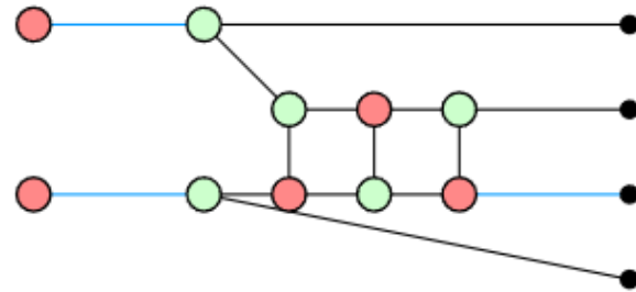
Figure 6.14: Simplified graph for row 3 and column 0.
