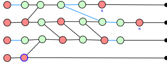
Figure 6.13: Visual representation of the orientation of edges for row 3 and column 0. Time flows from left to right.
