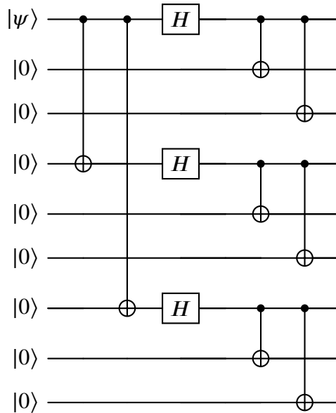
Figure 1.1: Shor Code circuit
