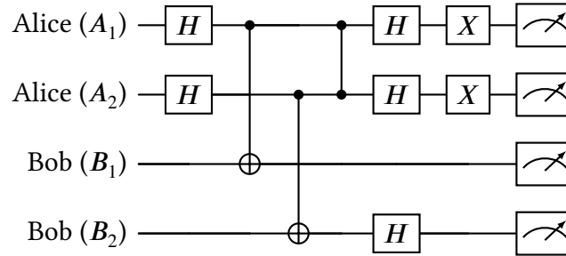
Figure 5.7: Mermin-Peres game circuit implementation for the first column and the third row.
