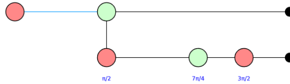
Figure 6.10: Simplification of the ZX diagram for the implementation of CHSH game, corresponding to (x, y) = (0, 0) , and with preparation of initial state in the computational basis.
