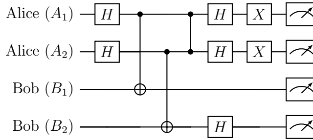
Figure 8: Mermin-Peres game circuit implementation for the first column and the third row.
