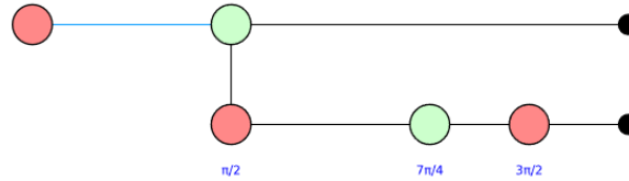
Figure 18: Simplification of the ZX diagram for the implementation of CHSH game, corresponding to (x, y) = (0, 0) , and with preparation of initial state in the computational basis.
