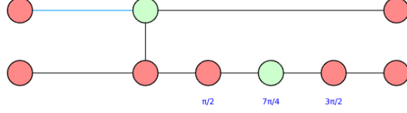
Figure 15: ZX diagram corresponding to (x, y) = (0, 0) and (m_0, m_1) = (0, 0)
