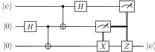
Figure 5: Standard quantum teleportation circuit.
