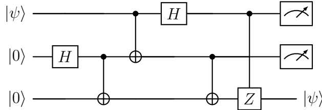
Figure 6: Standard quantum teleportation circuit without classical control.
