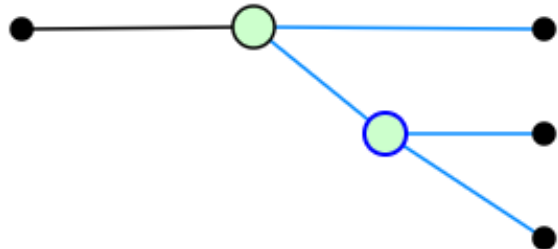
Figure 13: Simplified teleportation protocol without the classical control operations.
