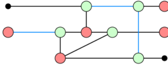
Figure 11: Simplification of the teleportation diagram when Alice measures (0, 0) .
