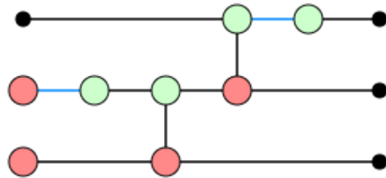
Figure 12: Teleportation protocol without the classical control operations.
