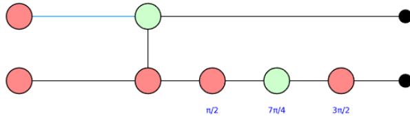
Figure 16: ZX diagram for the implementation of CHSH game, corresponding to (x, y) = (0, 0) .
