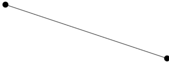
Figure 10: Identity channel resulting from the simplification of the teleportation diagrams
