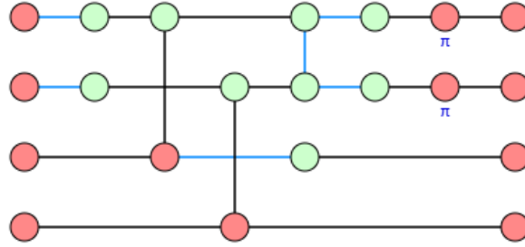
Figure 20: ZX diagram for row 3 and column 0 with boundary conditions corresponding to the covector \langle 0000| .
