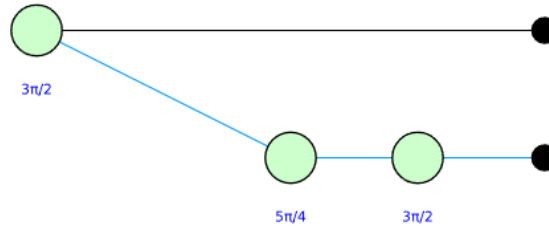
Figure 17: Simplification of the ZX diagram for the implementation of CHSH game, corresponding to (x, y) = (0, 0) .
