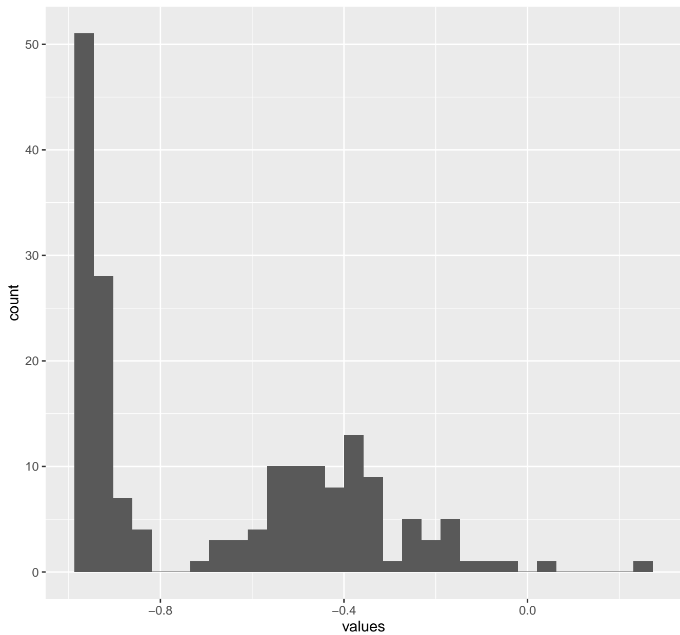
FrequencyBodyGyroscopeMagnitude.std..
