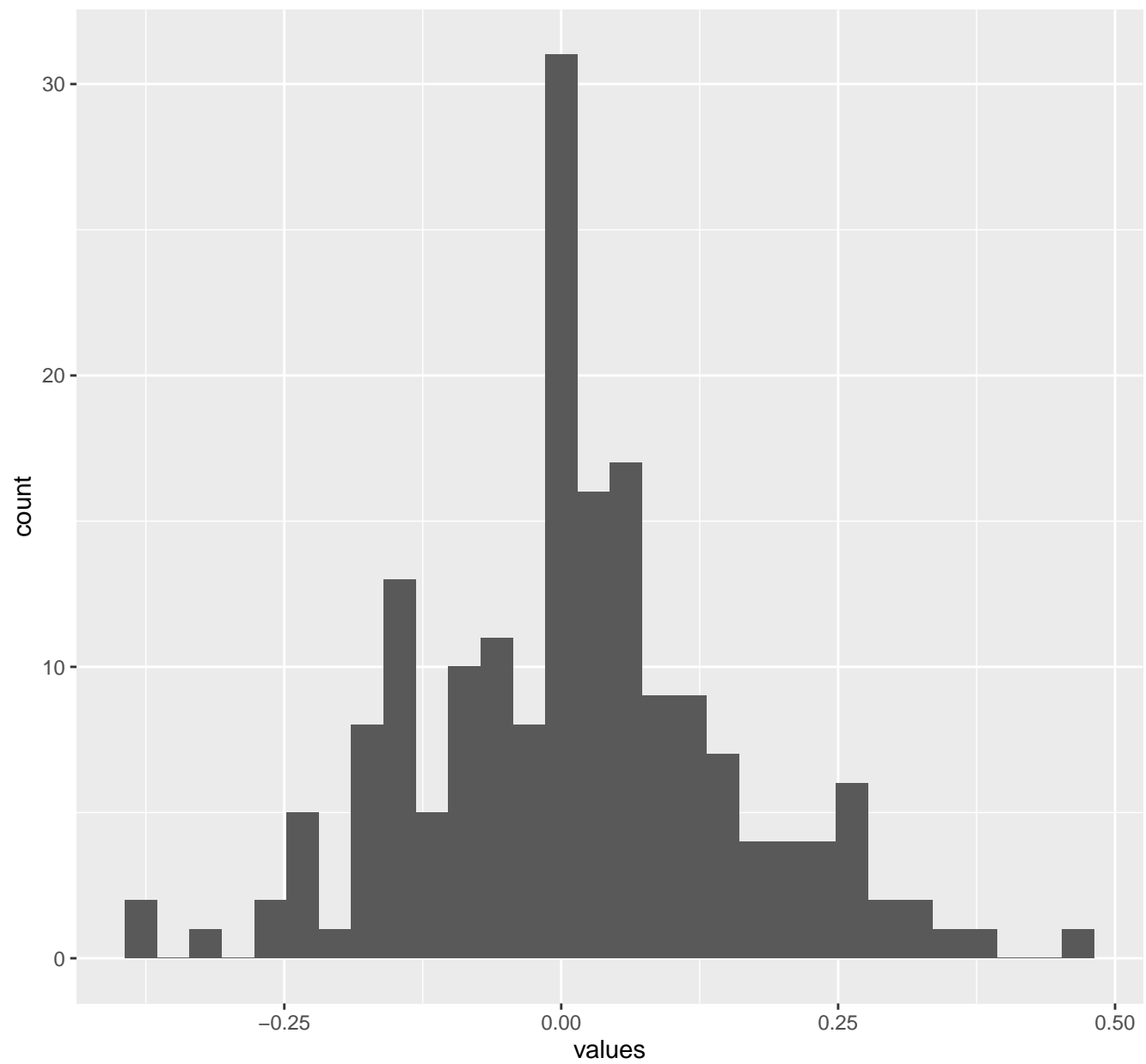
FrequencyBodyAccelerometer.meanFreq...Y
