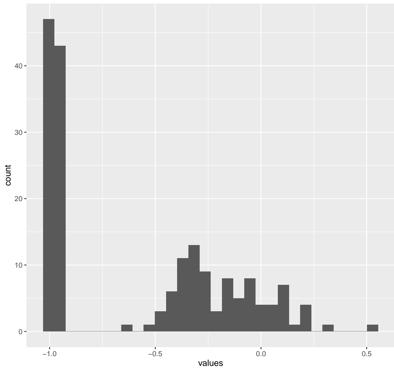
FrequencyBodyAccelerometer.mean...X
