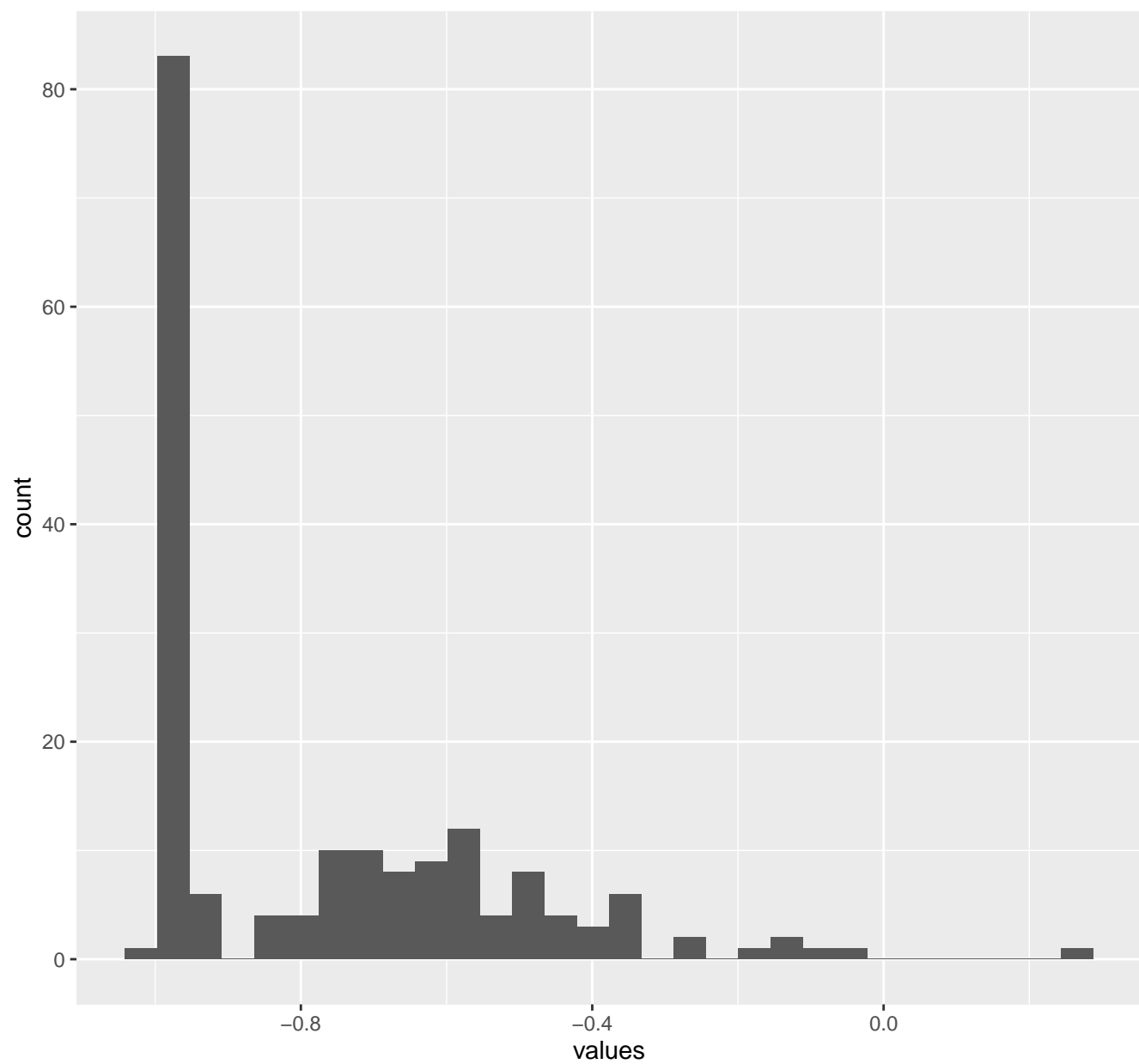
FrequencyBodyGyroscopeJerkMagnitude.std..
