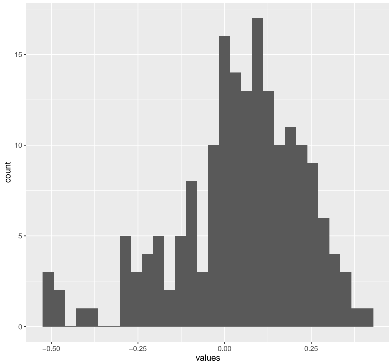
FrequencyBodyAccelerometer.meanFreq...Z
