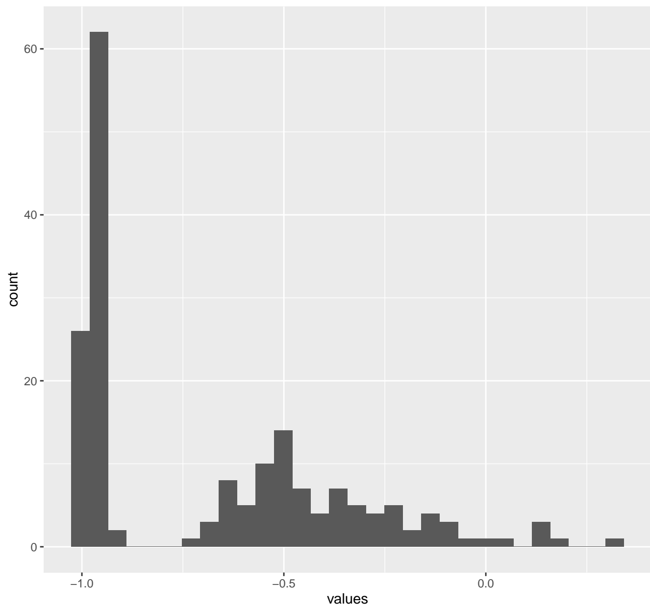
FrequencyBodyGyroscope.mean...Y
