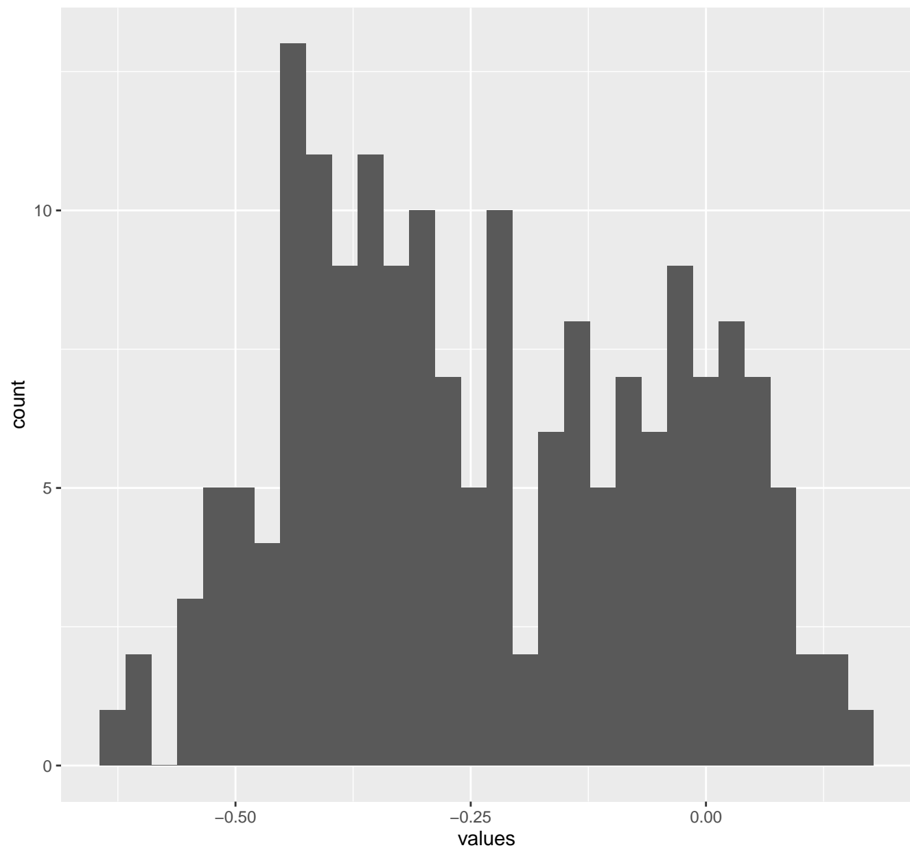
FrequencyBodyAccelerometer.meanFreq...X
