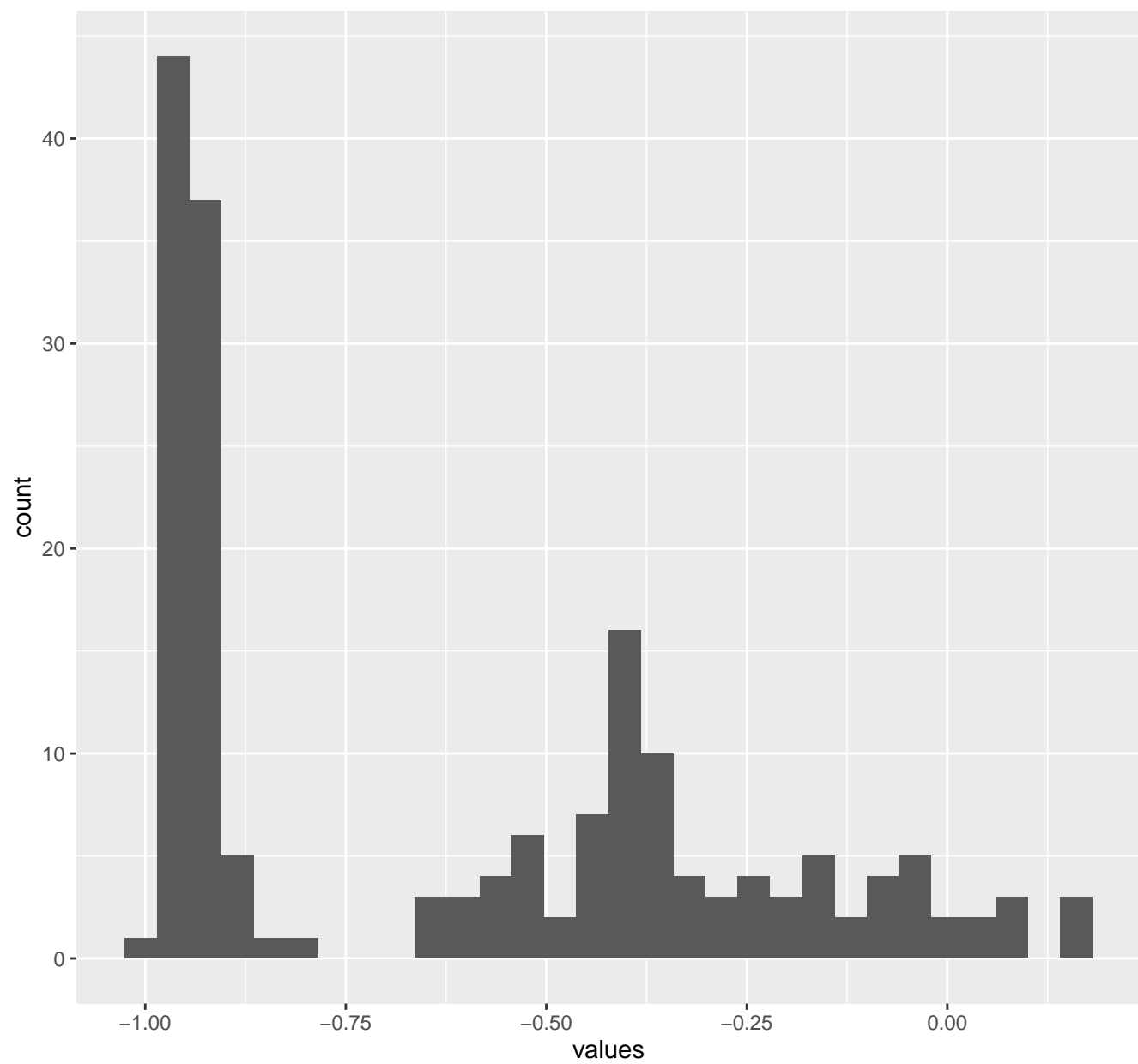
FrequencyBodyAccelerometerMagnitude.std..
