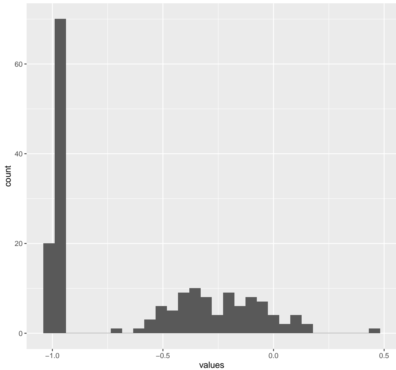
FrequencyBodyAccelerometerJerk.std...X
