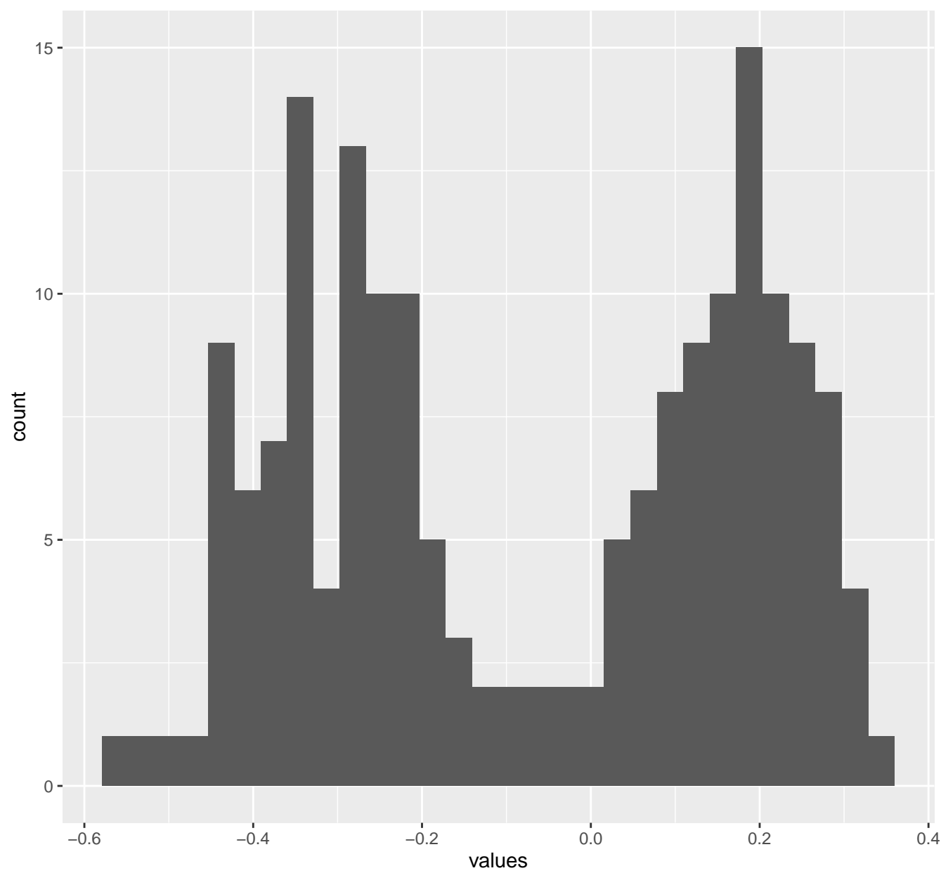
FrequencyBodyAccelerometerJerk.meanFreq...X
