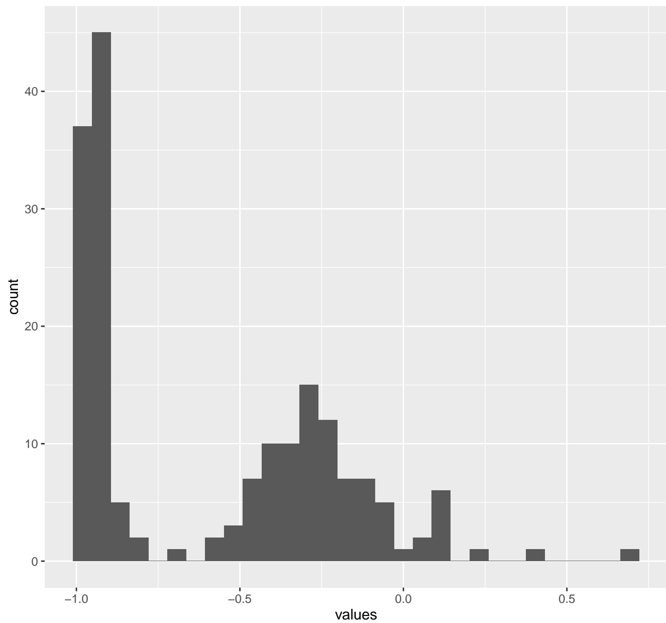
FrequencyBodyAccelerometer.std...Z
