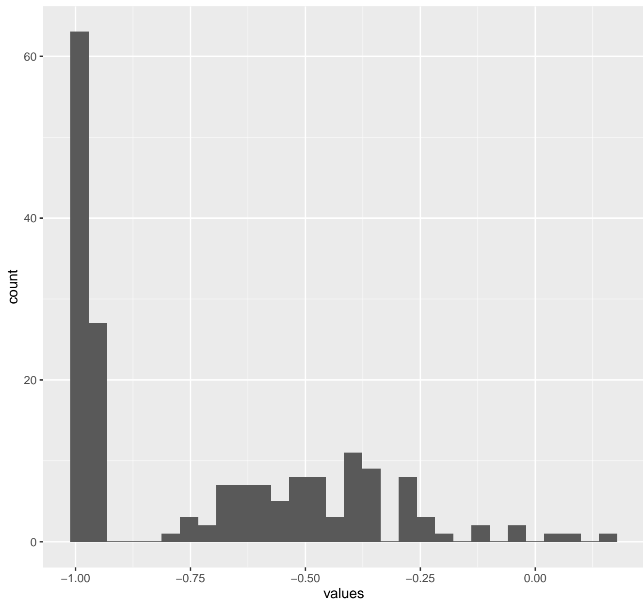
FrequencyBodyAccelerometerJerk.mean...Z
