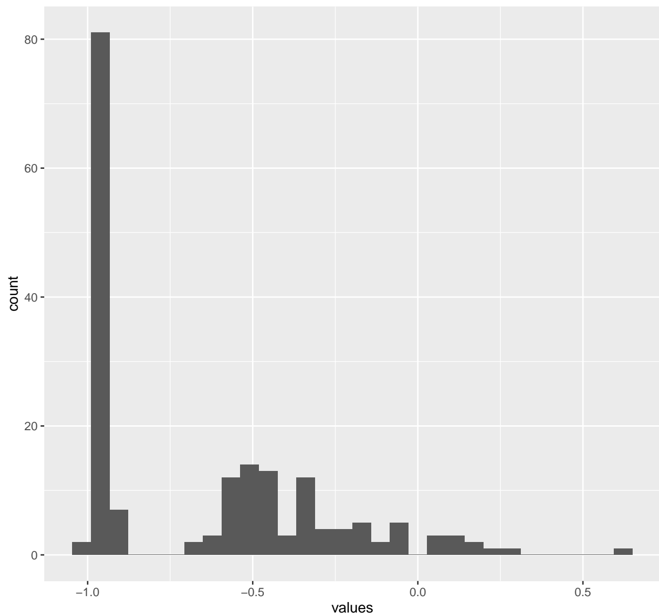
FrequencyBodyGyroscope.std...Y
