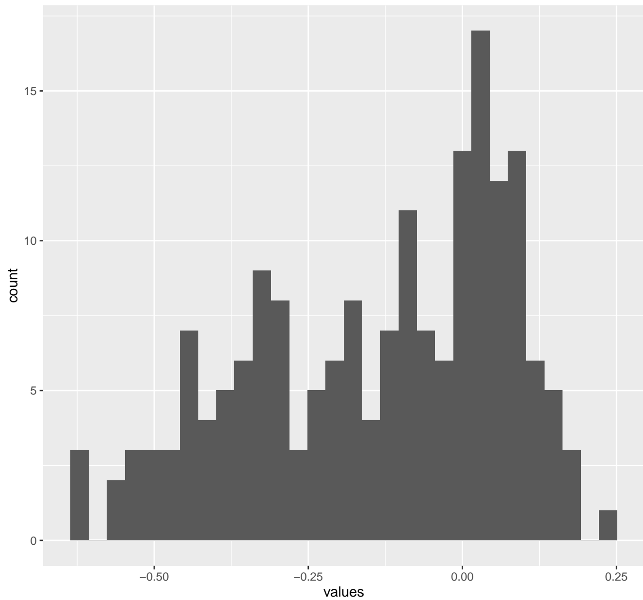
FrequencyBodyAccelerometerJerk.meanFreq...Z
