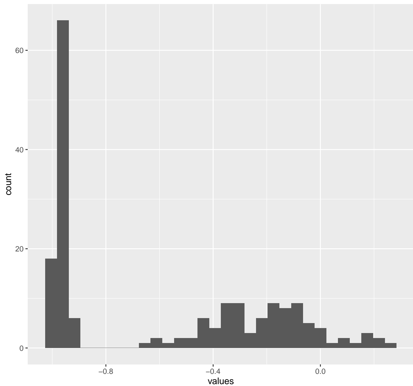
FrequencyBodyAccelerometerJerk.mean...Y
