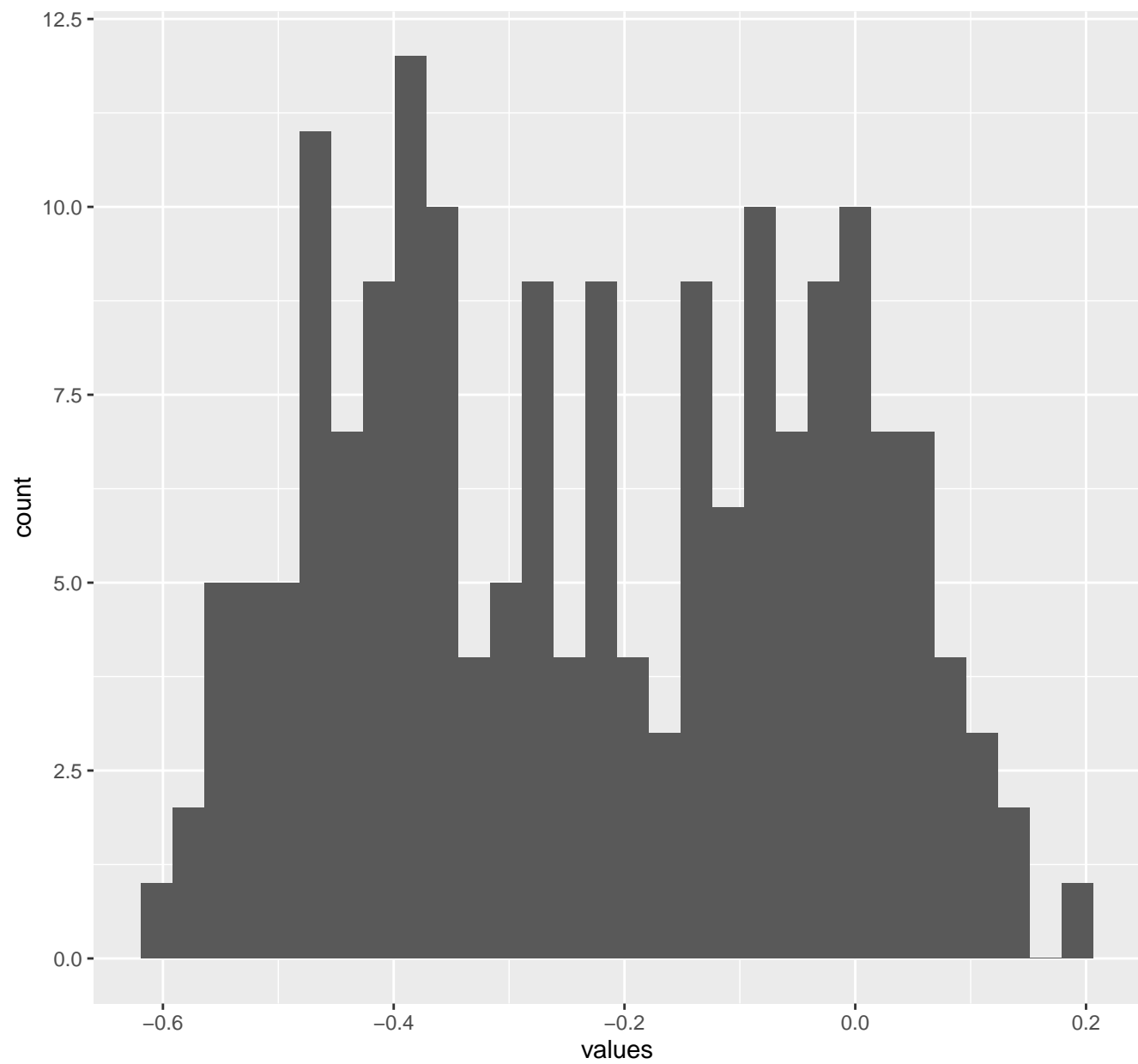
FrequencyBodyAccelerometerJerk.meanFreq...Y
