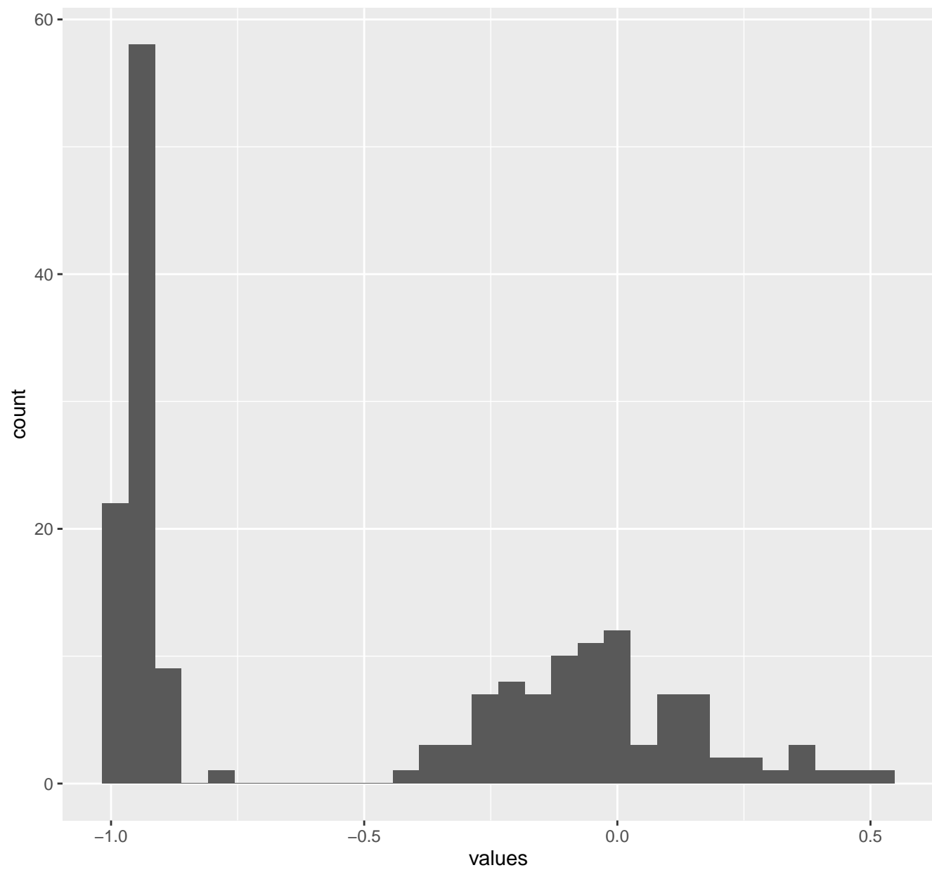
FrequencyBodyAccelerometer.mean...Y
