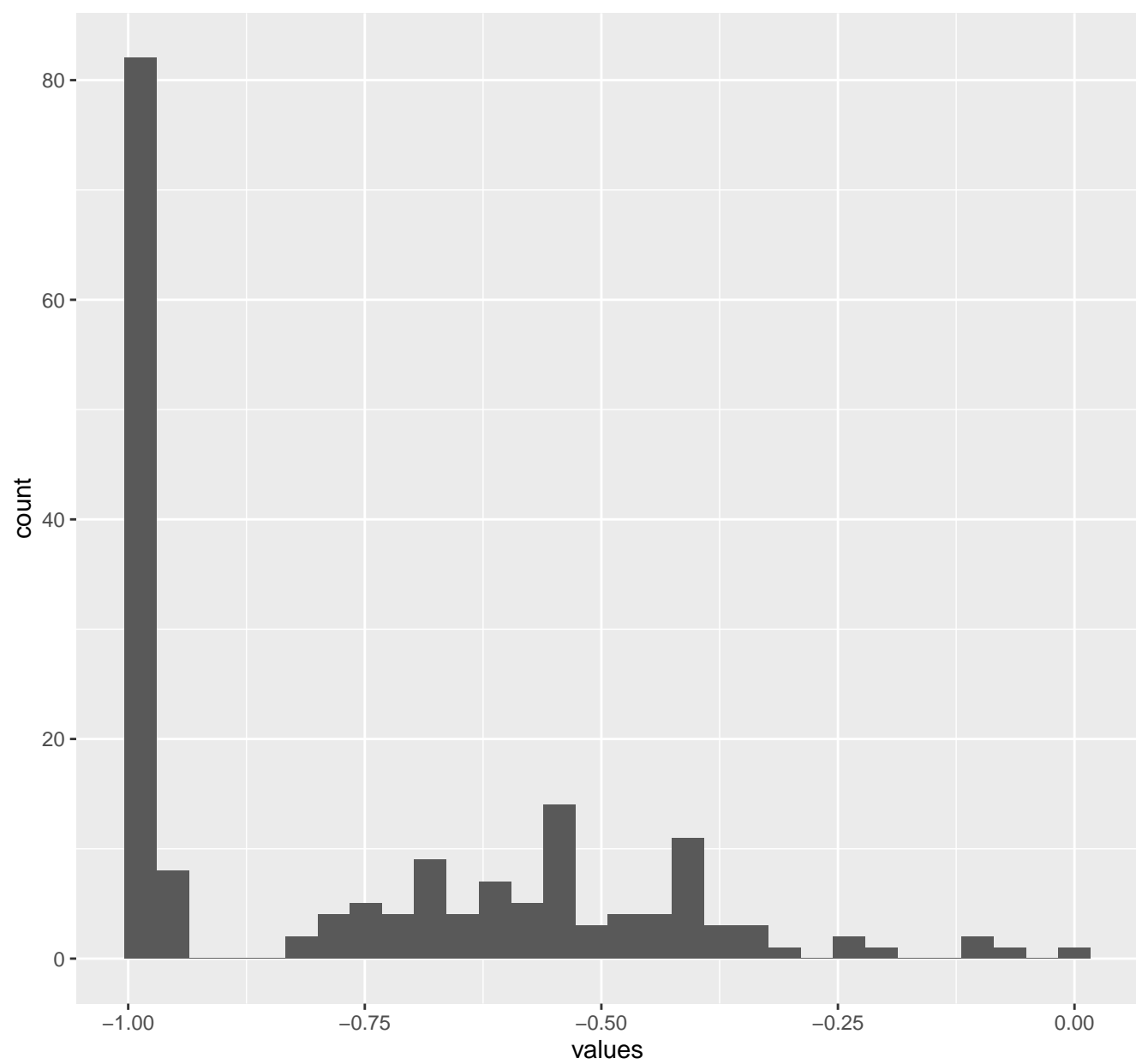
FrequencyBodyAccelerometerJerk.std...Z
