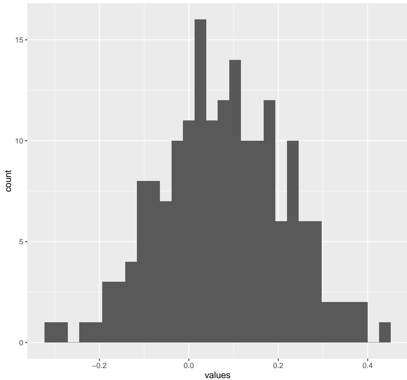
FrequencyBodyAccelerometerMagnitude.meanFreq..
