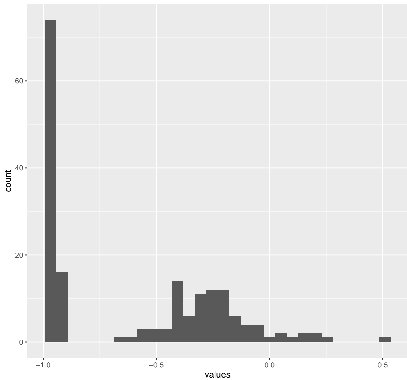
FrequencyBodyGyroscope.mean...Z
