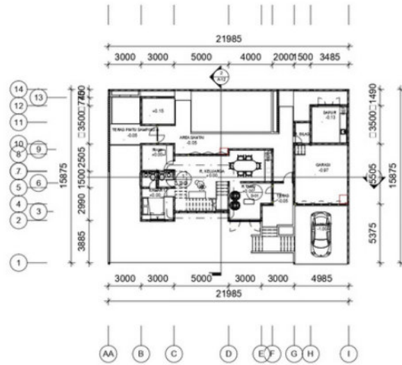
FLOOR PLAN 1
