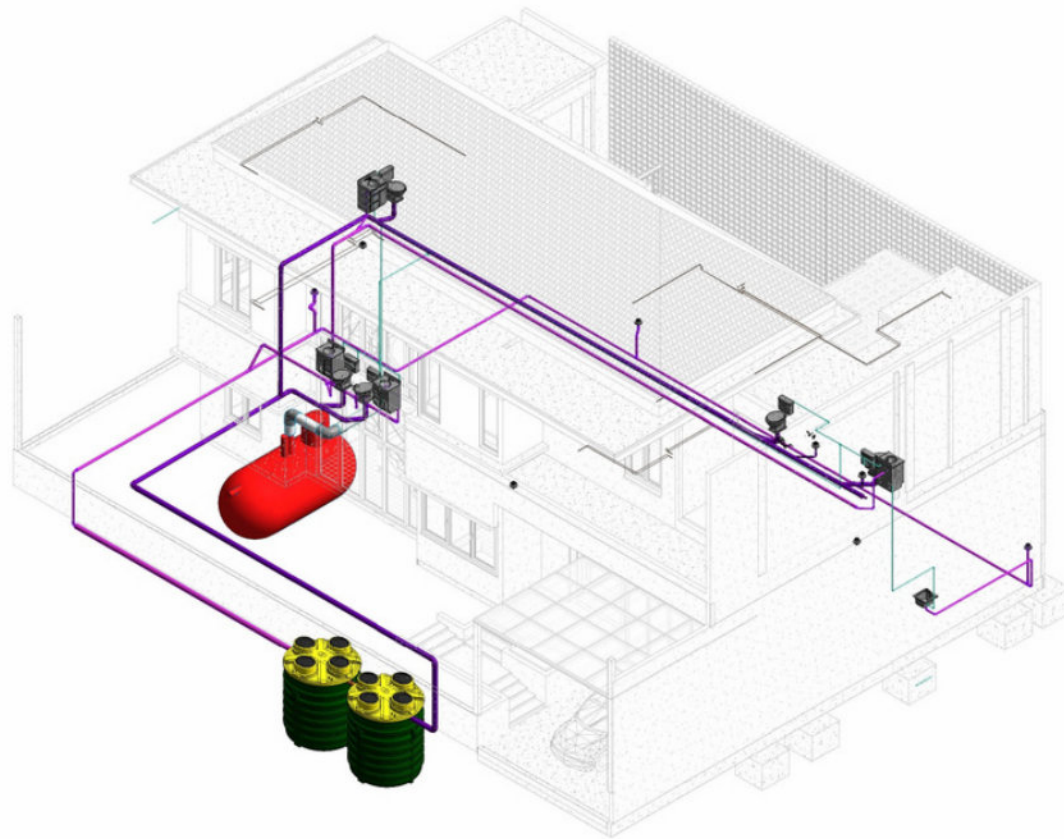
ISOMETRI PLUMBING
