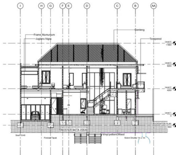
SECTION 1
