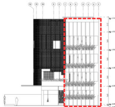
Left Elevation
