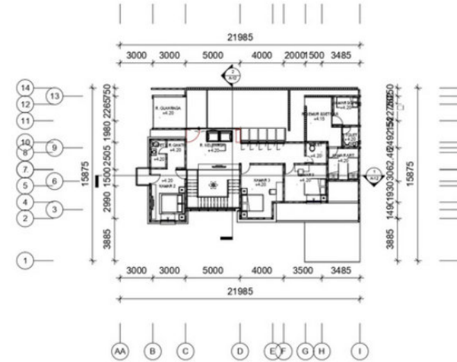
FLOOR PLAN 2
