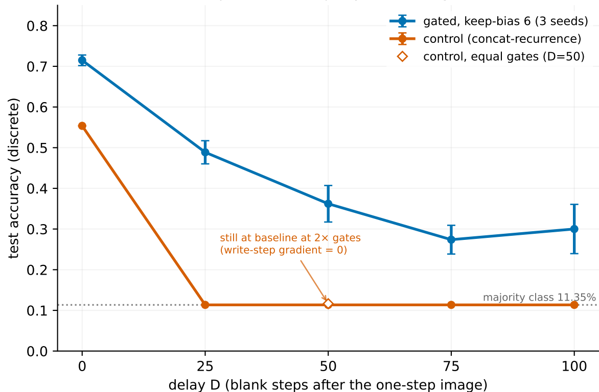
delayed-recall MNIST — accuracy vs delay (control collapses to the majority baseline · gated holds)
