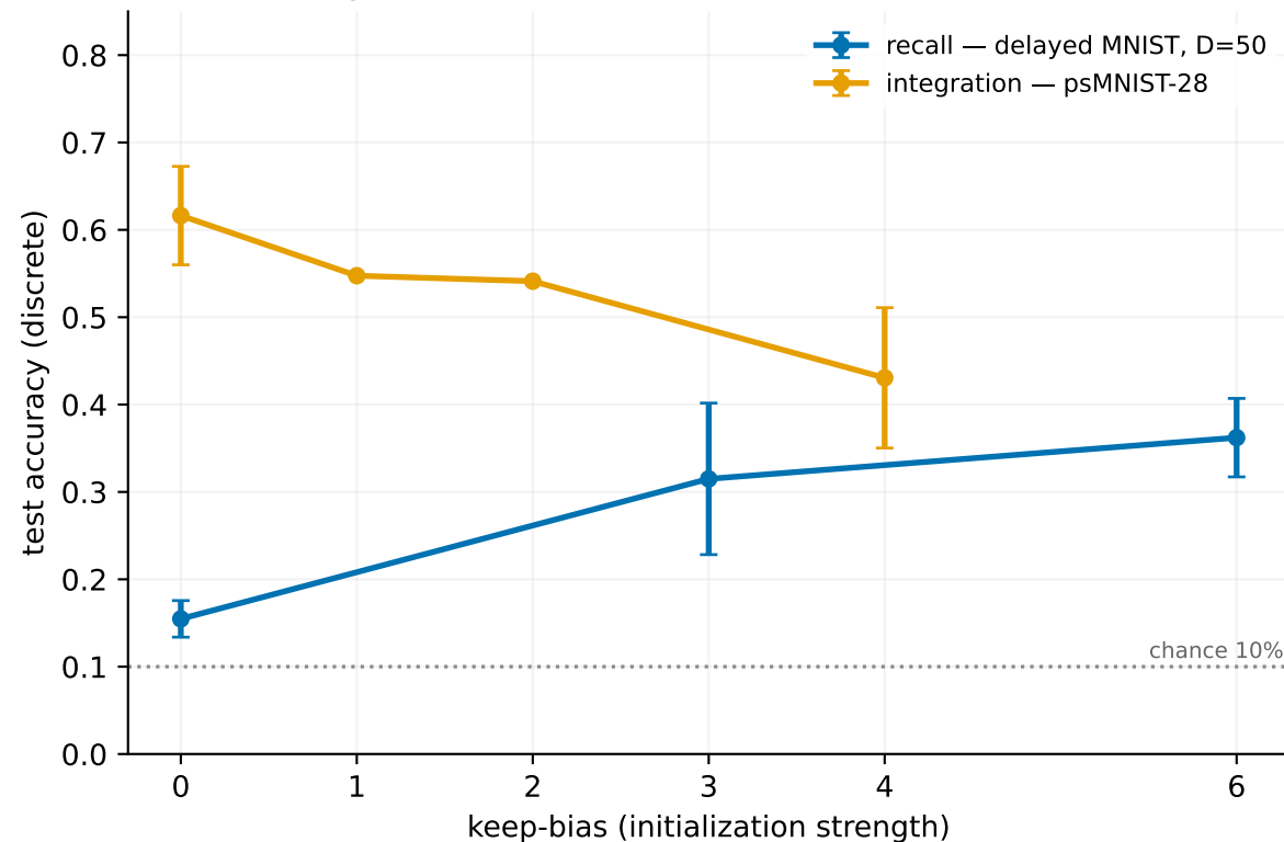
keep-bias is a task-dependent dial (high to HOLD · low to ABSORB; bars where 3 seeds)
