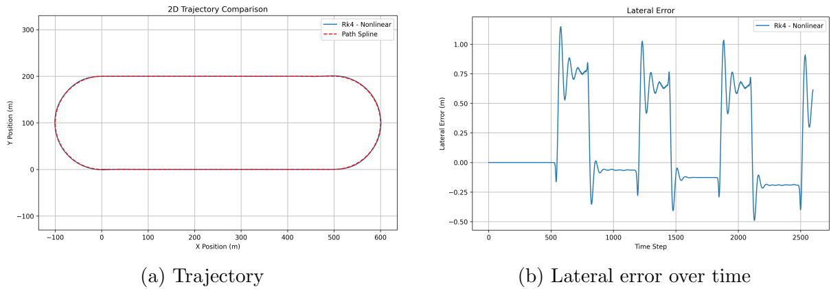
Figure 12: Kinematic MPC test at 25 m/s
