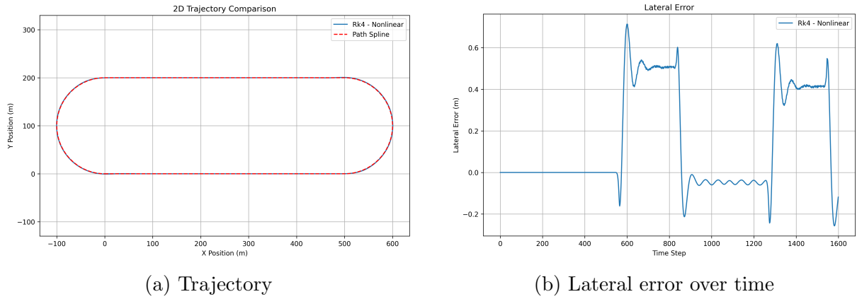
Figure 11: Kinematic MPC test at 23 m/s
