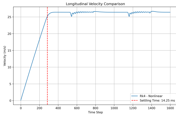
(a) Longitudinal Velocity
