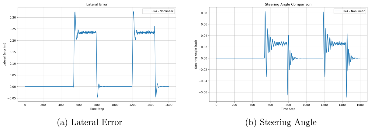
Figure 10: Pure Pursuit controller behavior at 25 m/s
